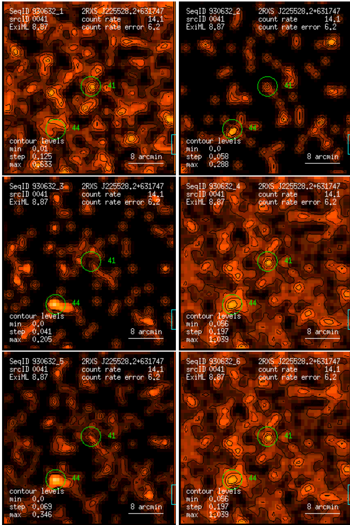
Figure 41: RASS 930632: detection 0041: band rate images, Gaussian filter: (1) PSPC channels 11 – 41, (2) 52 – 90, (3) 91 – 201, (4) 11 – 235, (5) 52 – 201, (6) 11 – 201. Broad band rates in counts/ks. Band rate contour levels in counts/ks/arcmin 2 .
