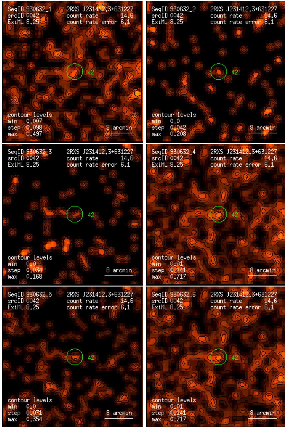
Figure 42: RASS 930632: detection 0042: band rate images, Gaussian filter: (1) PSPC channels 11 – 41, (2) 52 – 90, (3) 91 – 201, (4) 11 – 235, (5) 52 – 201, (6) 11 – 201. Broad band rates in counts/ks. Band rate contour levels in counts/ks/arcmin 2 .
