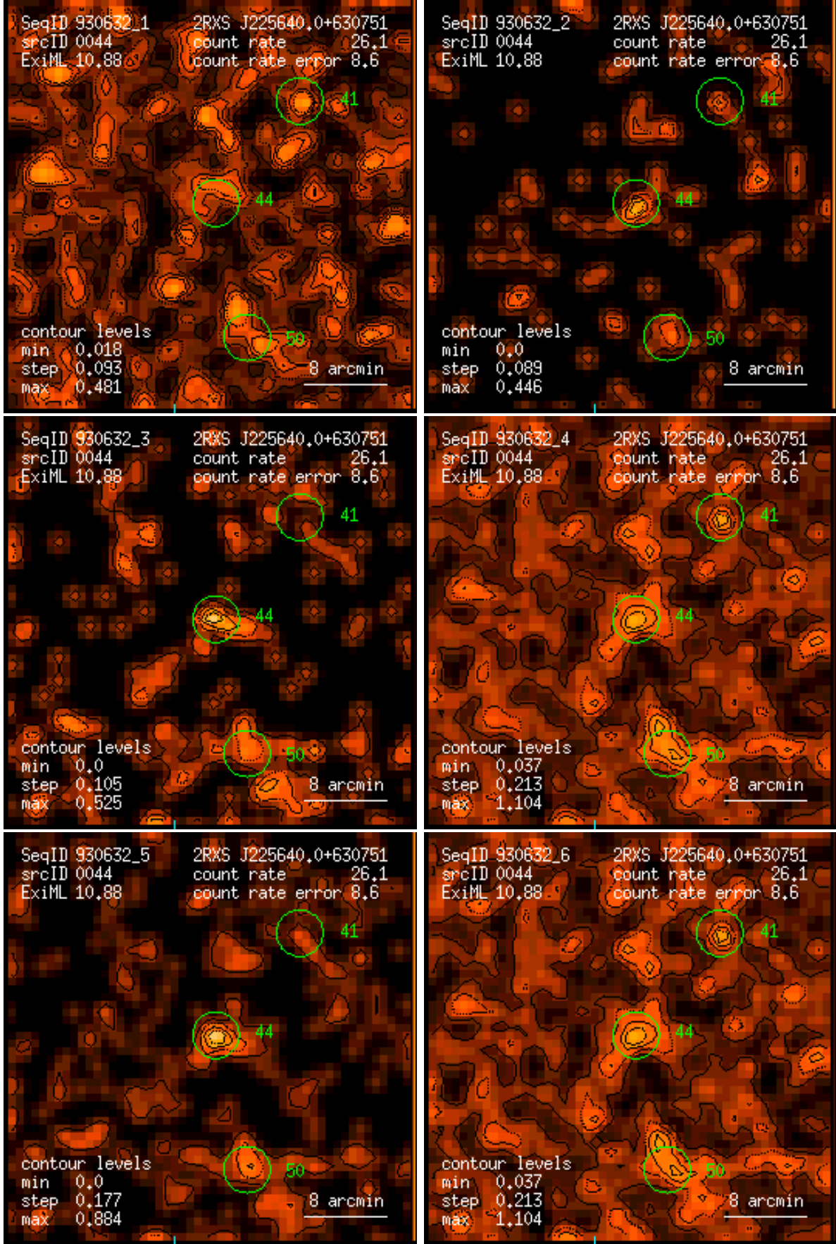
Figure 44: RASS 930632: detection 0044: band rate images, Gaussian filter: (1) PSPC channels 11 – 41, (2) 52 – 90, (3) 91 – 201, (4) 11 – 235, (5) 52 – 201, (6) 11 – 201. Broad band rates in counts/ks. Band rate contour levels in counts/ks/arcmin 2 .
