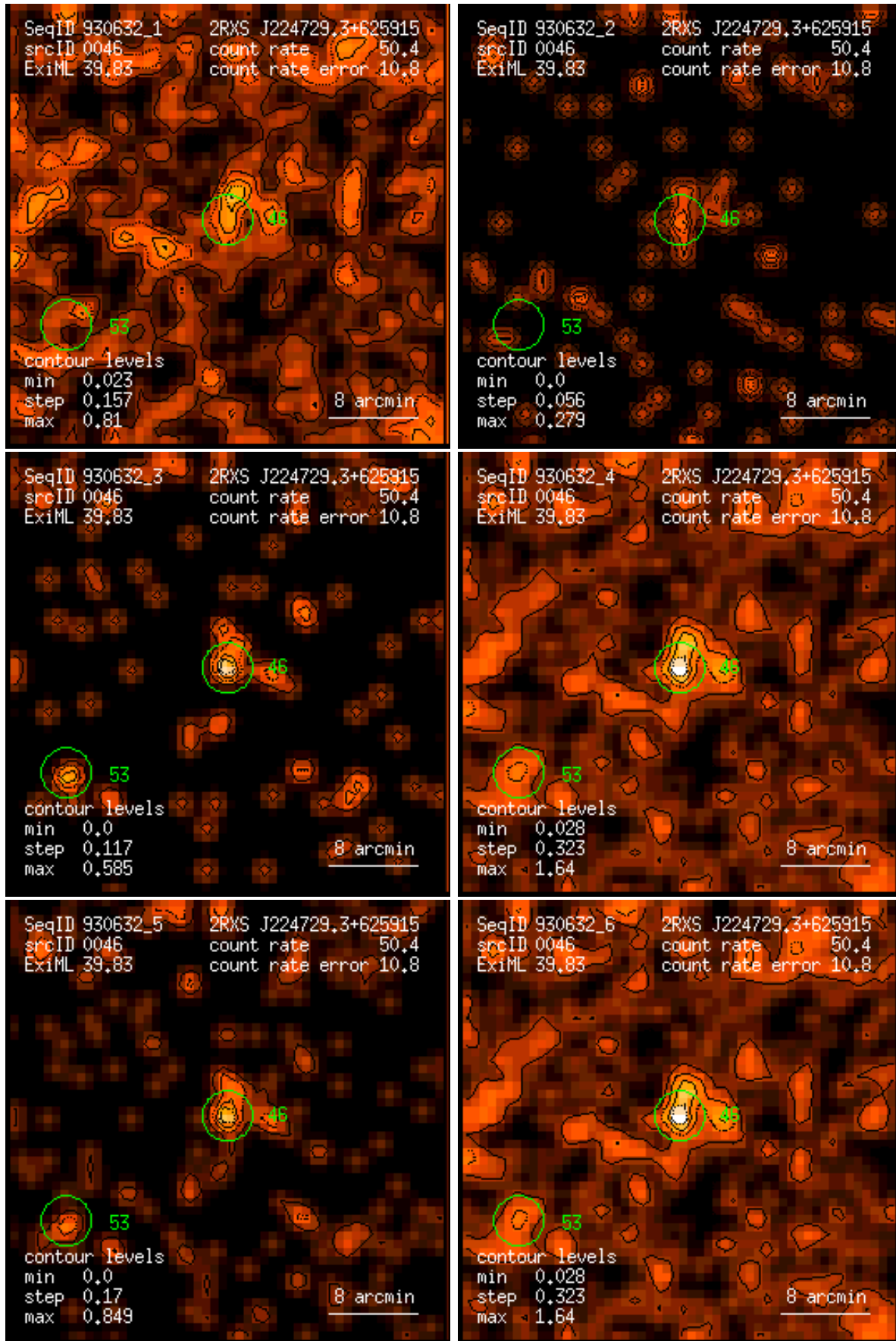
Figure 46: RASS 930632: detection 0046: band rate images, Gaussian filter: (1) PSPC channels 11 – 41, (2) 52 – 90, (3) 91 – 201, (4) 11 – 235, (5) 52 – 201, (6) 11 – 201. Broad band rates in counts/ks. Band rate contour levels in counts/ks/arcmin 2 .
