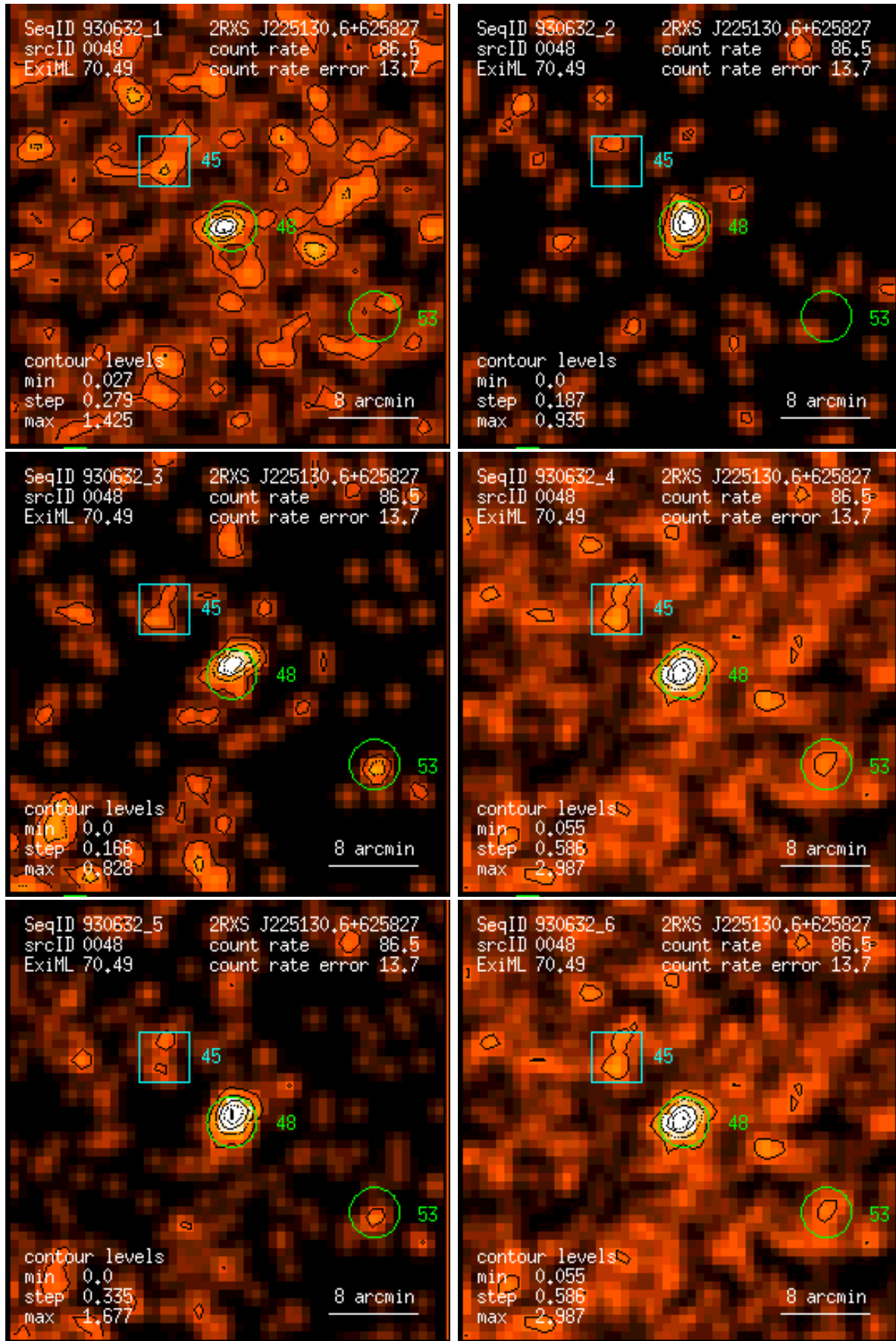
Figure 48: RASS 930632: detection 0048: band rate images, Gaussian filter: (1) PSPC channels 11 – 41, (2) 52 – 90, (3) 91 – 201, (4) 11 – 235, (5) 52 – 201, (6) 11 – 201. Broad band rates in counts/ks. Band rate contour levels in counts/ks/arcmin 2 .
