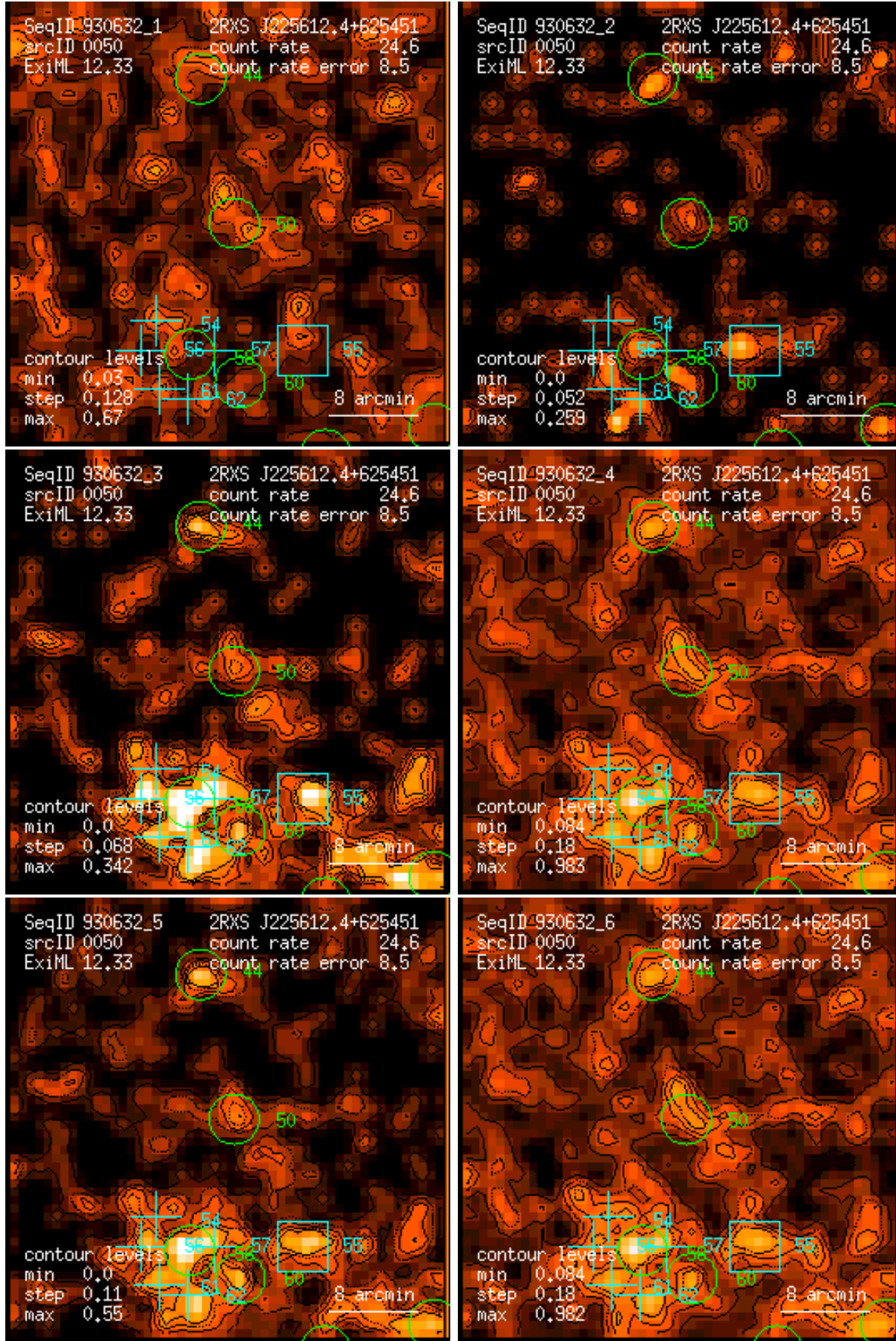
Figure 50: RASS 930632: detection 0050: band rate images, Gaussian filter: (1) PSPC channels 11 – 41, (2) 52 – 90, (3) 91 – 201, (4) 11 – 235, (5) 52 – 201, (6) 11 – 201. Broad band rates in counts/ks. Band rate contour levels in counts/ks/arcmin 2 .
