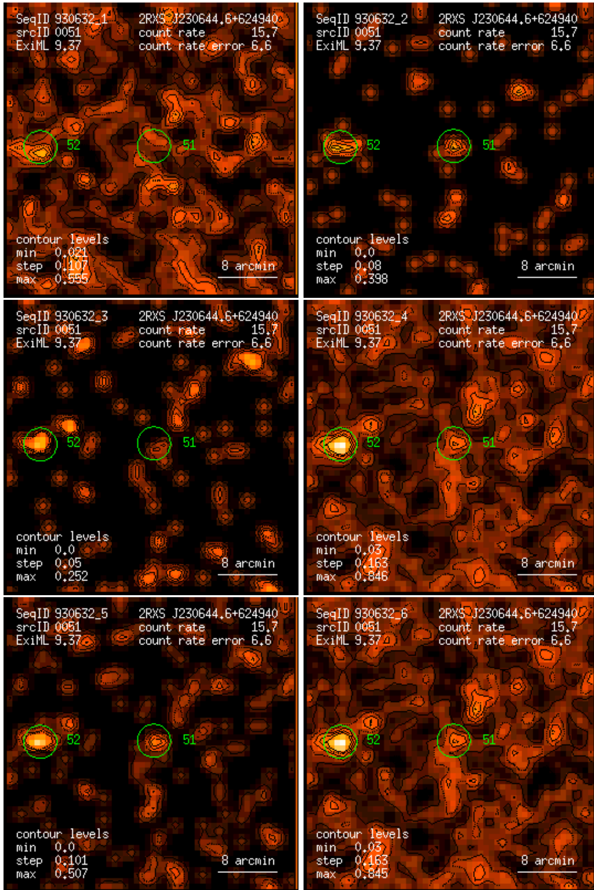
Figure 51: RASS 930632: detection 0051: band rate images, Gaussian filter: (1) PSPC channels 11 – 41, (2) 52 – 90, (3) 91 – 201, (4) 11 – 235, (5) 52 – 201, (6) 11 – 201. Broad band rates in counts/ks. Band rate contour levels in counts/ks/arcmin 2 .
