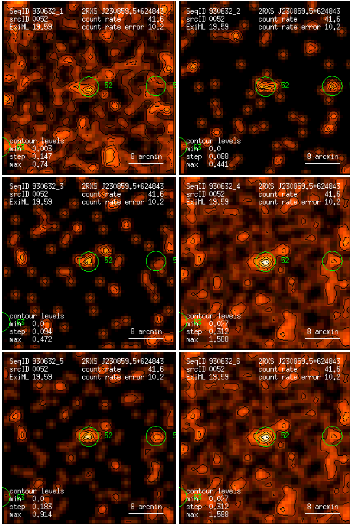
Figure 52: RASS 930632: detection 0052: band rate images, Gaussian filter: (1) PSPC channels 11 – 41, (2) 52 – 90, (3) 91 – 201, (4) 11 – 235, (5) 52 – 201, (6) 11 – 201. Broad band rates in counts/ks. Band rate contour levels in counts/ks/arcmin 2 .
