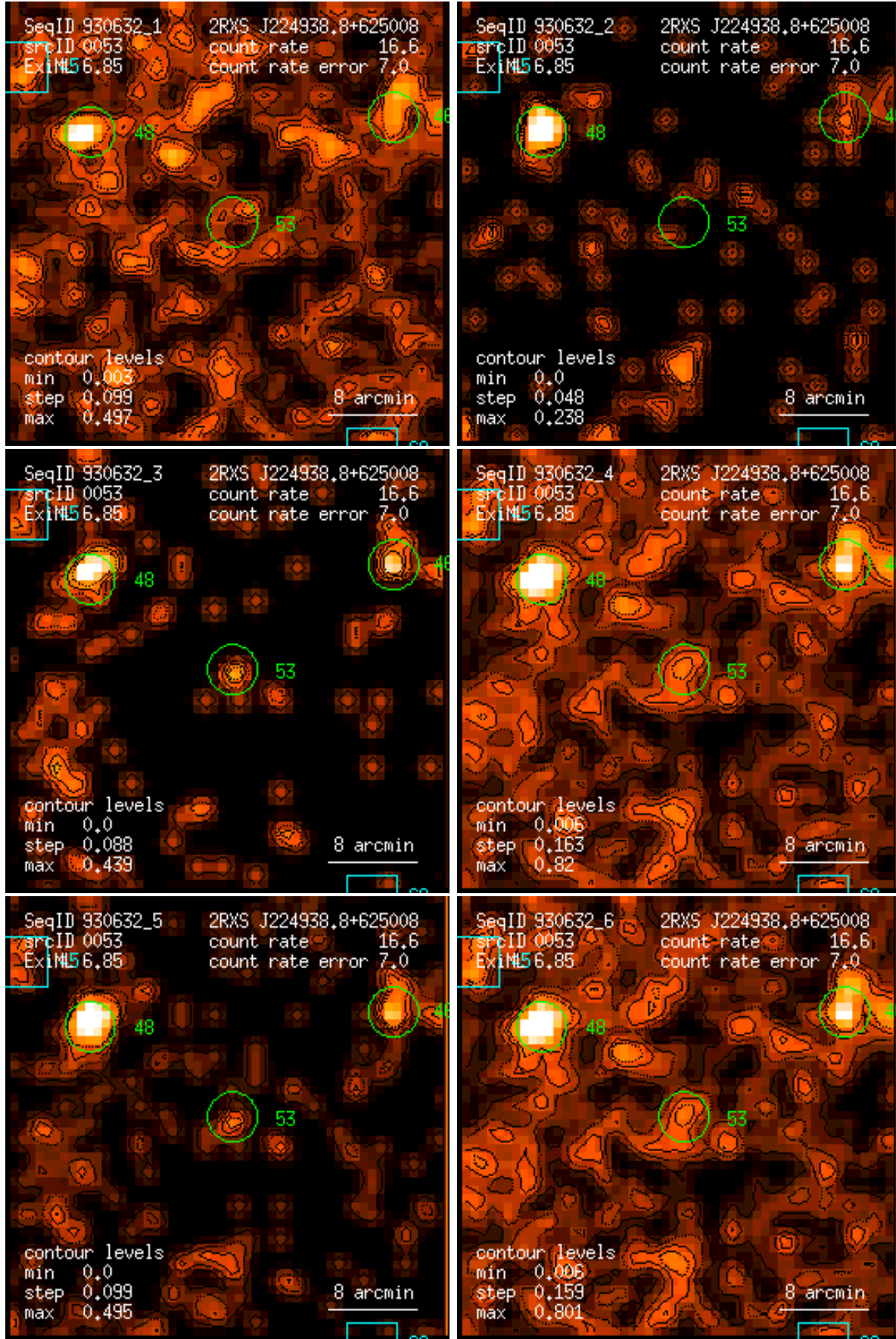
Figure 53: RASS 930632: detection 0053: band rate images, Gaussian filter: (1) PSPC channels 11 – 41, (2) 52 – 90, (3) 91 – 201, (4) 11 – 235, (5) 52 – 201, (6) 11 – 201. Broad band rates in counts/ks. Band rate contour levels in counts/ks/arcmin 2 .
