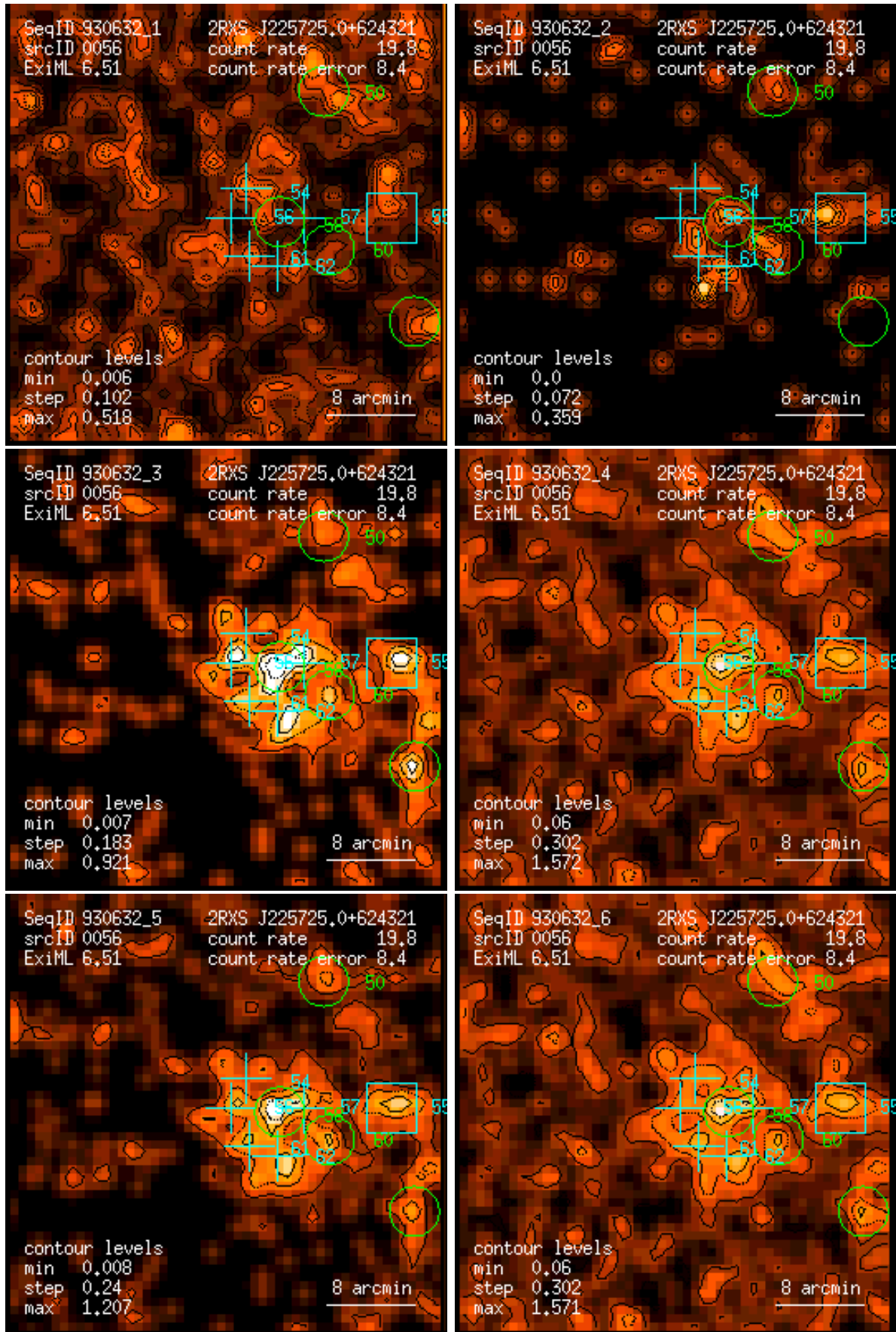
Figure 56: RASS 930632: detection 0056: band rate images, Gaussian filter: (1) PSPC channels 11 – 41, (2) 52 – 90, (3) 91 – 201, (4) 11 – 235, (5) 52 – 201, (6) 11 – 201. Broad band rates in counts/ks. Band rate contour levels in counts/ks/arcmin 2 .
