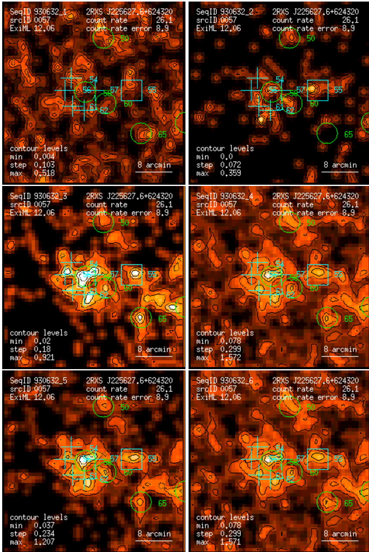
Figure 57: RASS 930632: detection 0057: band rate images, Gaussian filter: (1) PSPC channels 11 – 41, (2) 52 – 90, (3) 91 – 201, (4) 11 – 235, (5) 52 – 201, (6) 11 – 201. Broad band rates in counts/ks. Band rate contour levels in counts/ks/arcmin 2 .
