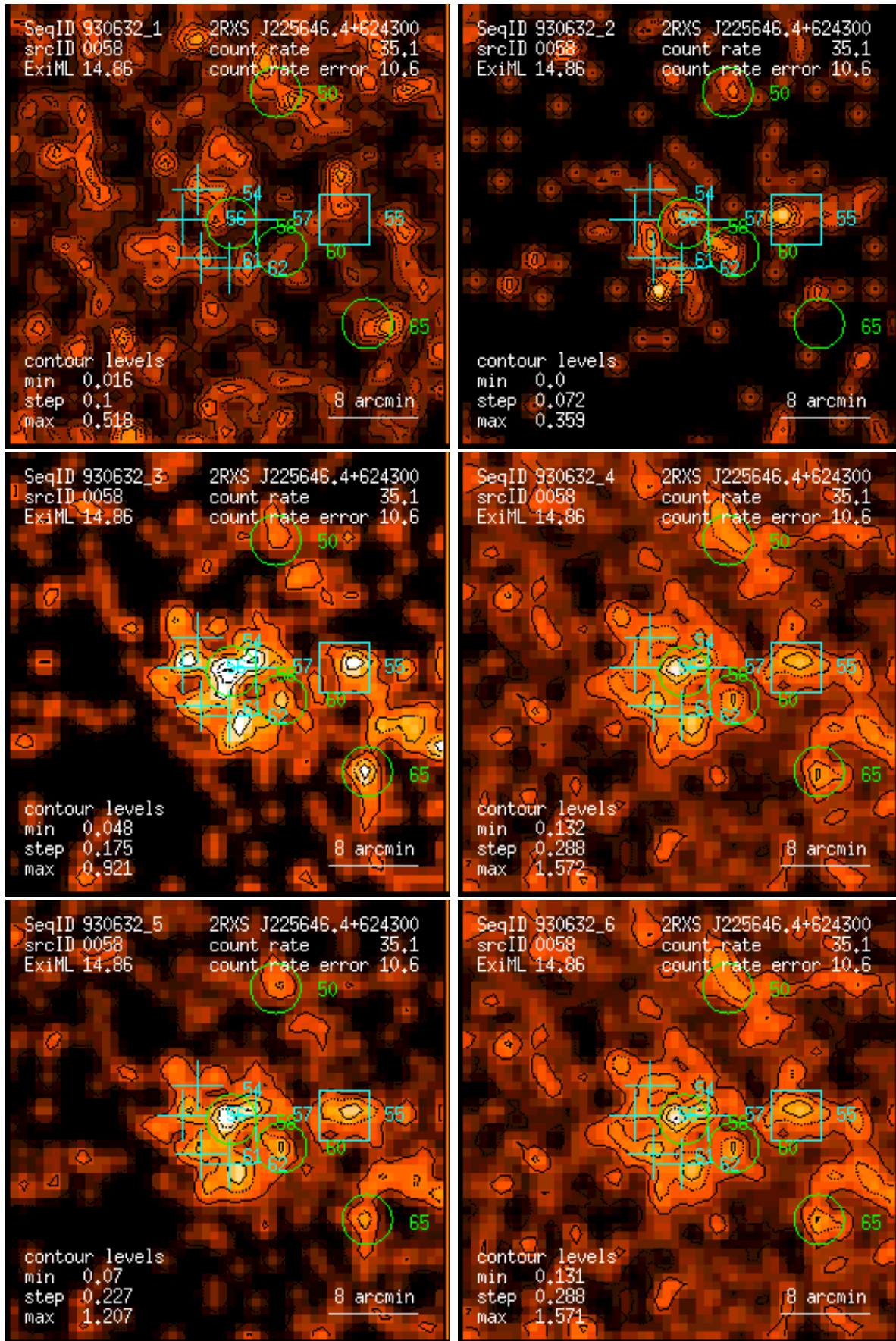
Figure 58: RASS 930632: detection 0058: band rate images, Gaussian filter: (1) PSPC channels 11 – 41, (2) 52 – 90, (3) 91 – 201, (4) 11 – 235, (5) 52 – 201, (6) 11 – 201. Broad band rates in counts/ks. Band rate contour levels in counts/ks/arcmin 2 .
