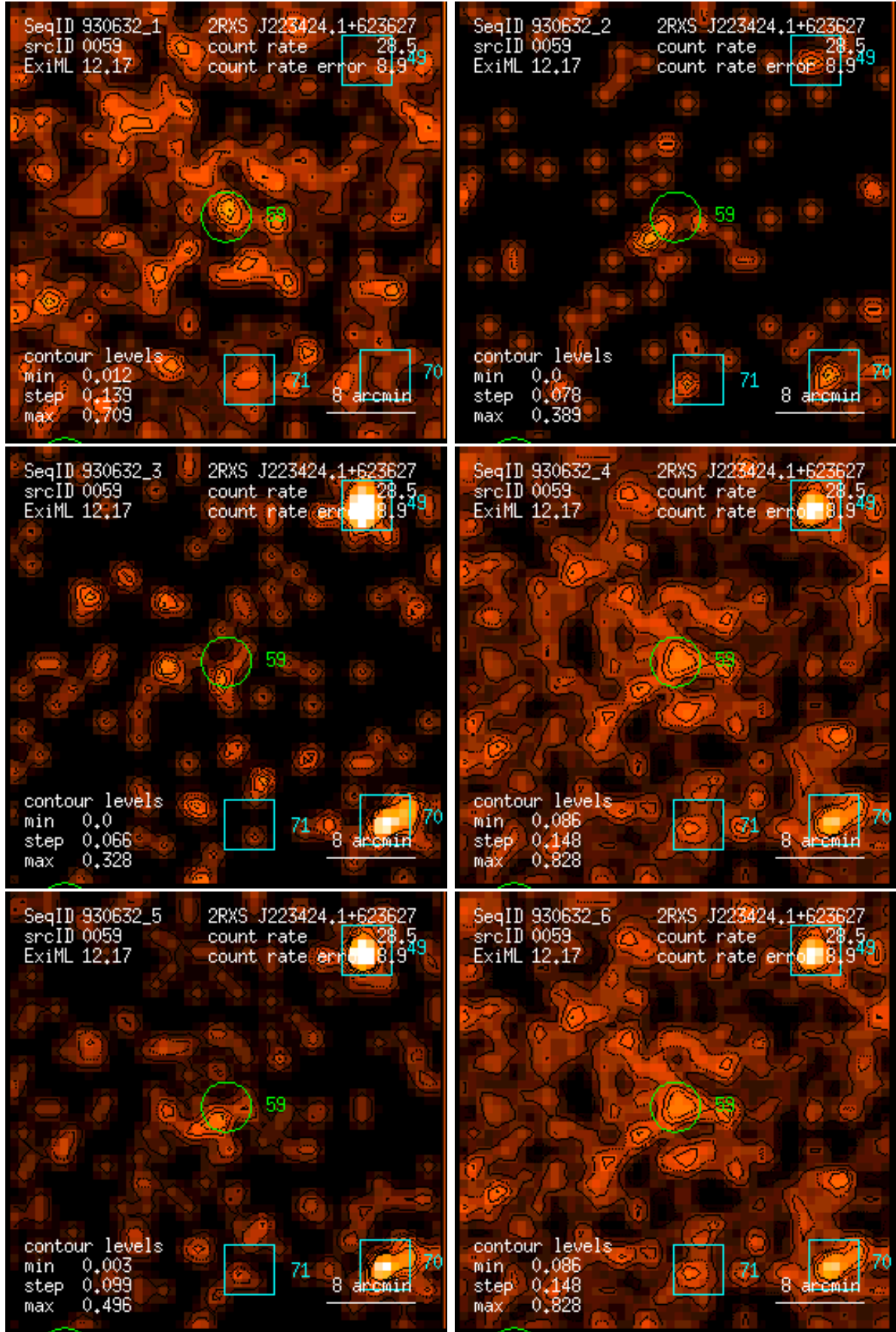
Figure 59: RASS 930632: detection 0059: band rate images, Gaussian filter: (1) PSPC channels 11 – 41, (2) 52 – 90, (3) 91 – 201, (4) 11 – 235, (5) 52 – 201, (6) 11 – 201. Broad band rates in counts/ks. Band rate contour levels in counts/ks/arcmin 2 .
