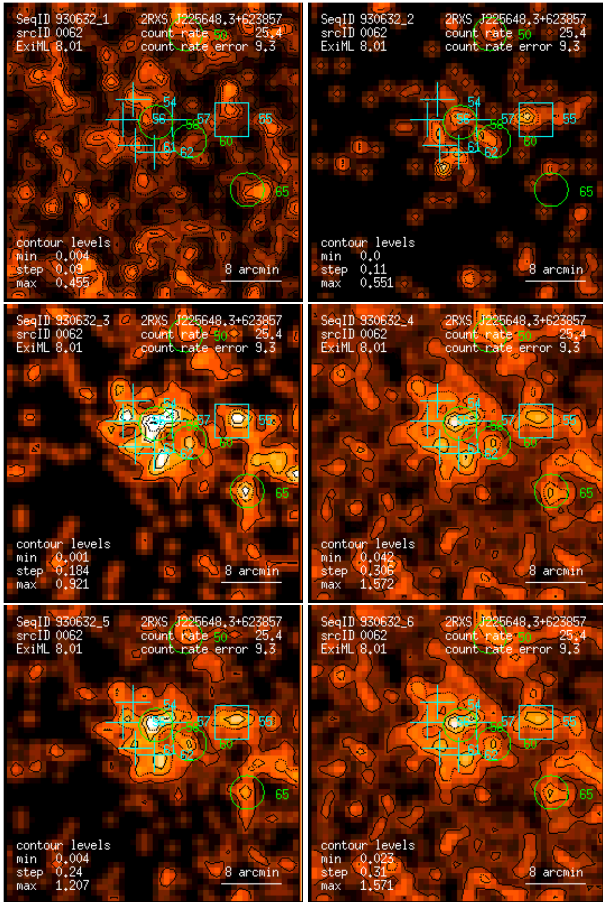
Figure 62: RASS 930632: detection 0062: band rate images, Gaussian filter: (1) PSPC channels 11 – 41, (2) 52 – 90, (3) 91 – 201, (4) 11 – 235, (5) 52 – 201, (6) 11 – 201. Broad band rates in counts/ks. Band rate contour levels in counts/ks/arcmin 2 .
