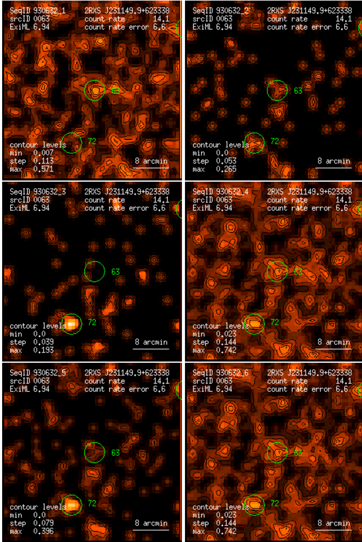
Figure 63: RASS 930632: detection 0063: band rate images, Gaussian filter: (1) PSPC channels 11 – 41, (2) 52 – 90, (3) 91 – 201, (4) 11 – 235, (5) 52 – 201, (6) 11 – 201. Broad band rates in counts/ks. Band rate contour levels in counts/ks/arcmin 2 .
