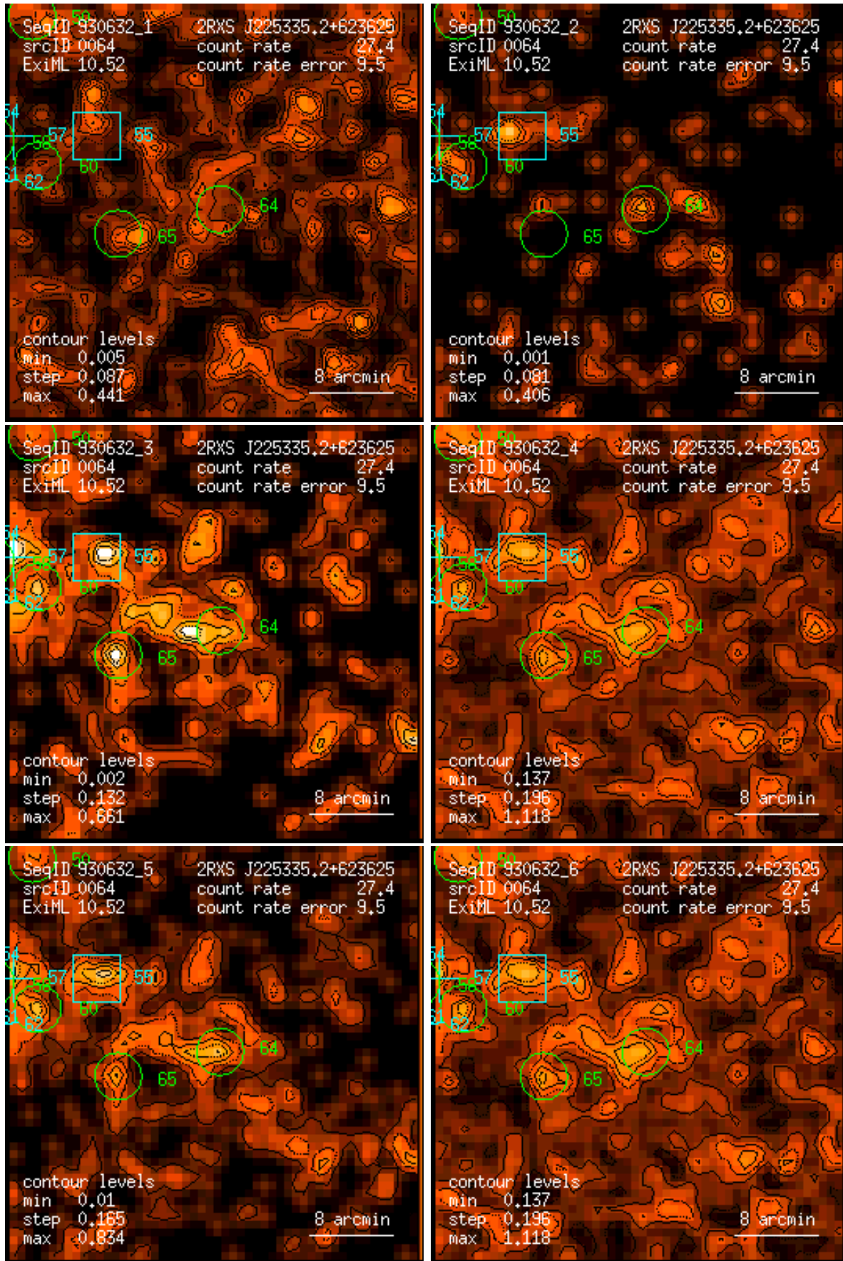
Figure 64: RASS 930632: detection 0064: band rate images, Gaussian filter: (1) PSPC channels 11 – 41, (2) 52 – 90, (3) 91 – 201, (4) 11 – 235, (5) 52 – 201, (6) 11 – 201. Broad band rates in counts/ks. Band rate contour levels in counts/ks/arcmin 2 .
