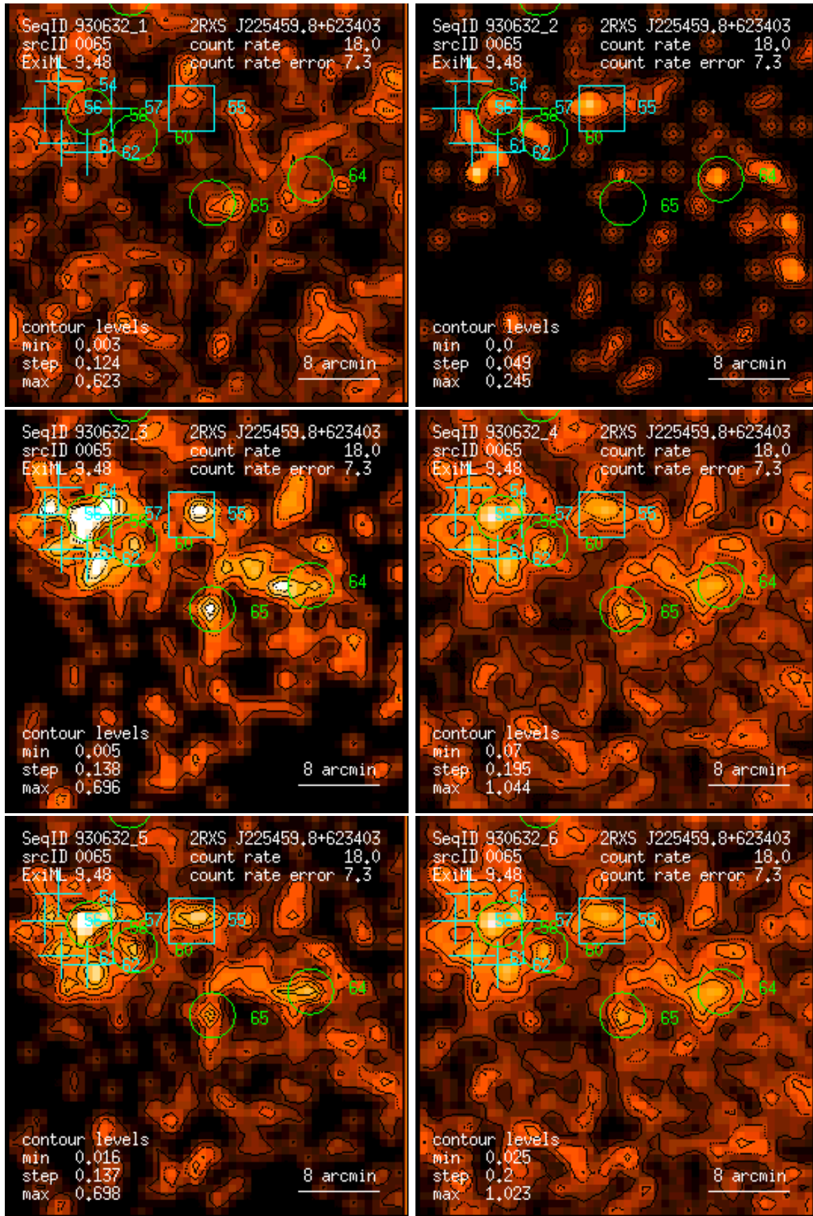
Figure 65: RASS 930632: detection 0065: band rate images, Gaussian filter: (1) PSPC channels 11 – 41, (2) 52 – 90, (3) 91 – 201, (4) 11 – 235, (5) 52 – 201, (6) 11 – 201. Broad band rates in counts/ks. Band rate contour levels in counts/ks/arcmin 2 .
