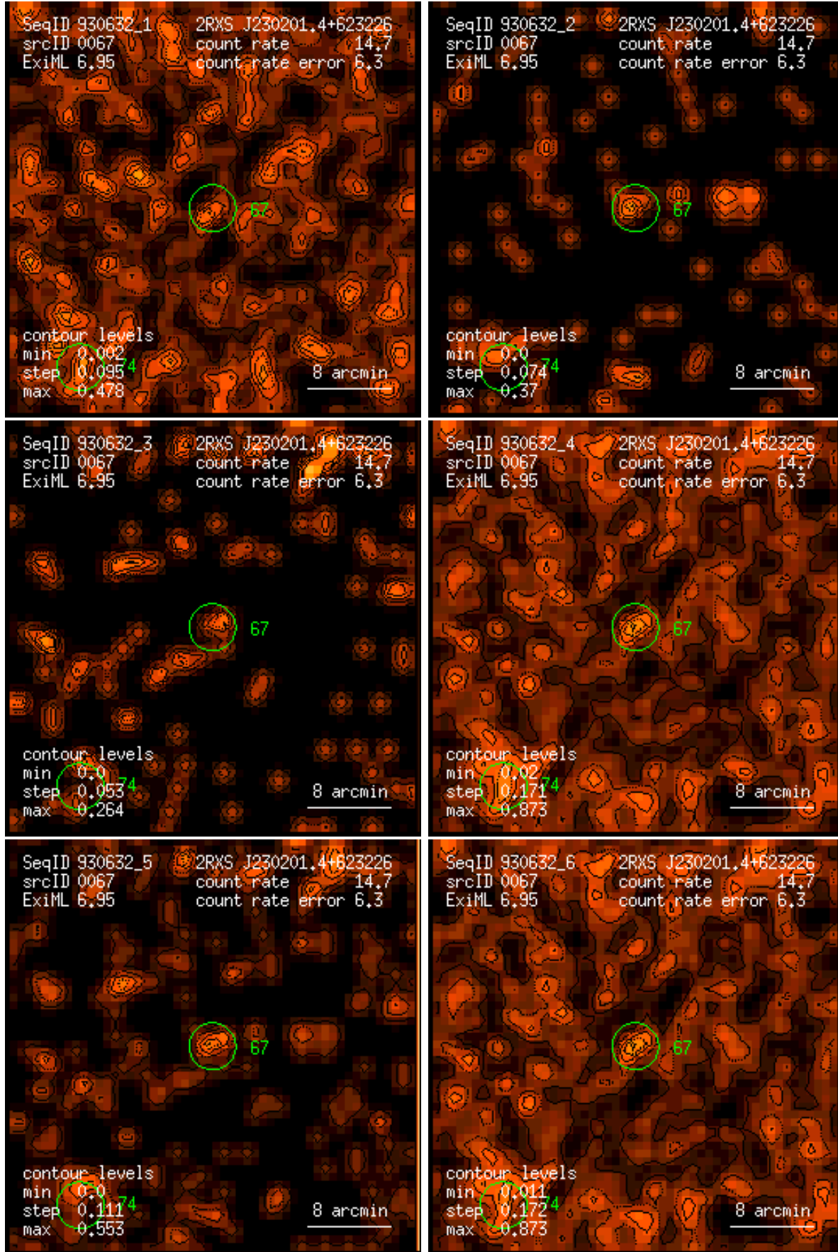
Figure 67: RASS 930632: detection 0067: band rate images, Gaussian filter: (1) PSPC channels 11 – 41, (2) 52 – 90, (3) 91 – 201, (4) 11 – 235, (5) 52 – 201, (6) 11 – 201. Broad band rates in counts/ks. Band rate contour levels in counts/ks/arcmin 2 .
