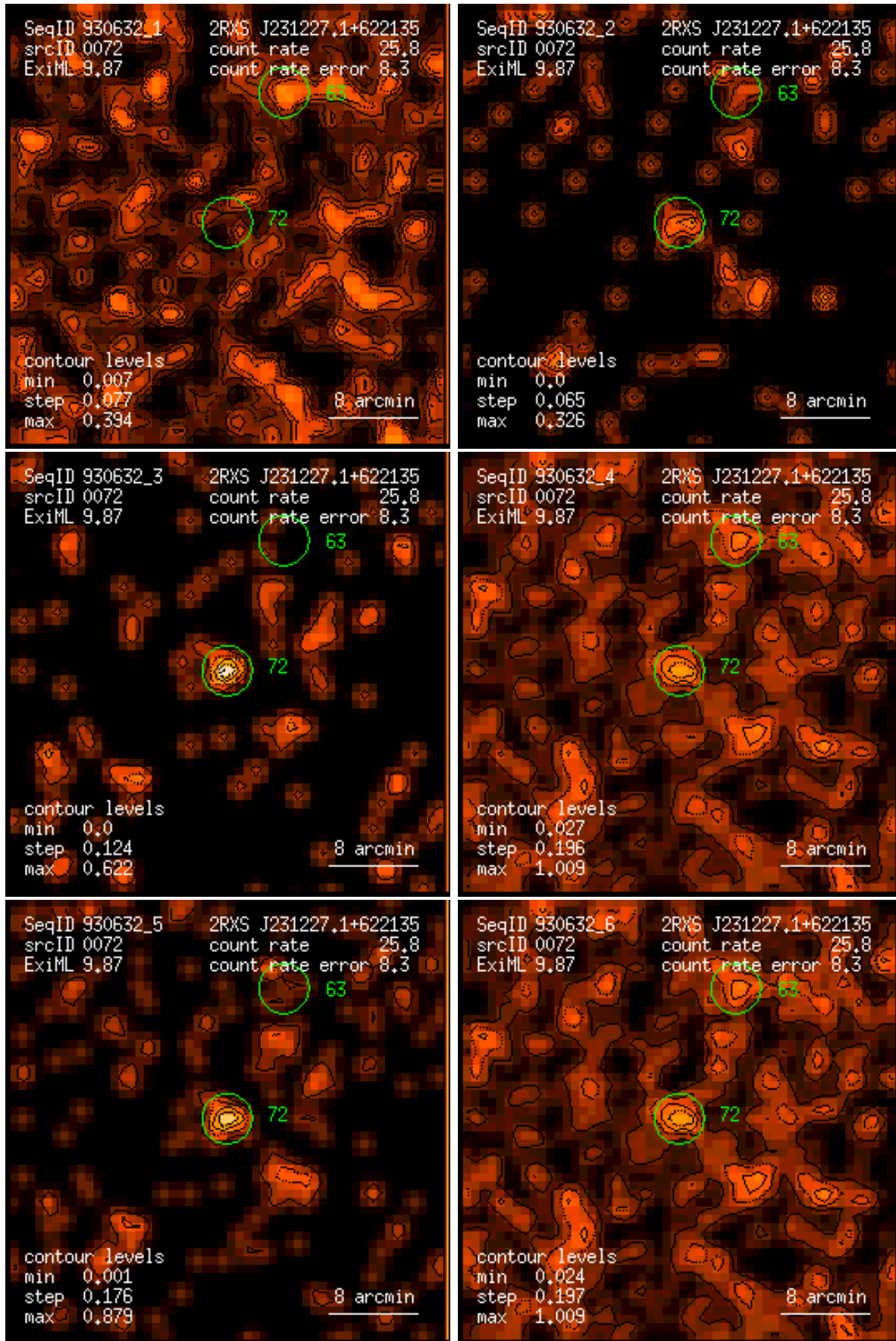
Figure 72: RASS 930632: detection 0072: band rate images, Gaussian filter: (1) PSPC channels 11 – 41, (2) 52 – 90, (3) 91 – 201, (4) 11 – 235, (5) 52 – 201, (6) 11 – 201. Broad band rates in counts/ks. Band rate contour levels in counts/ks/arcmin 2 .
