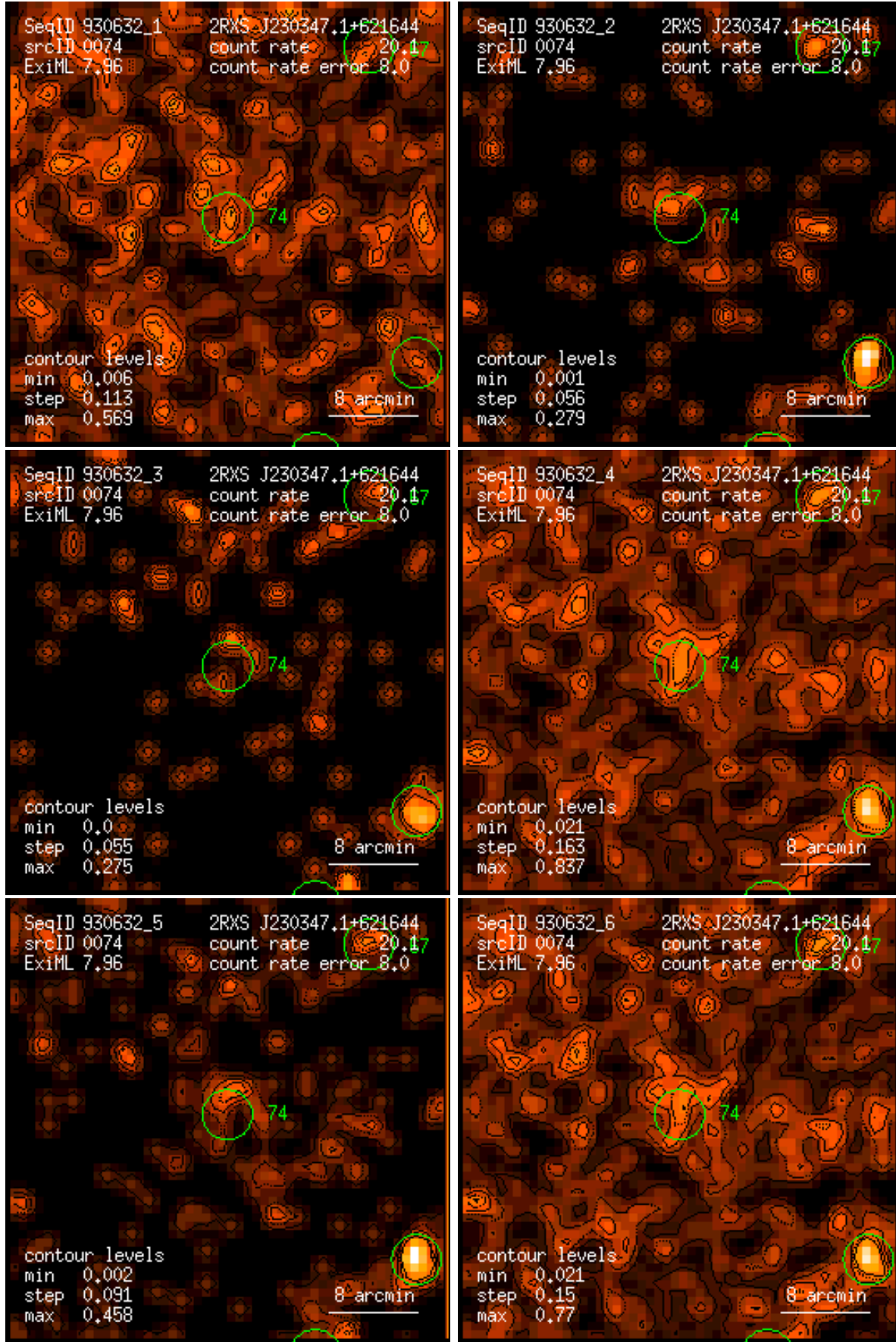
Figure 74: RASS 930632: detection 0074: band rate images, Gaussian filter: (1) PSPC channels 11 – 41, (2) 52 – 90, (3) 91 – 201, (4) 11 – 235, (5) 52 – 201, (6) 11 – 201. Broad band rates in counts/ks. Band rate contour levels in counts/ks/arcmin 2 .
