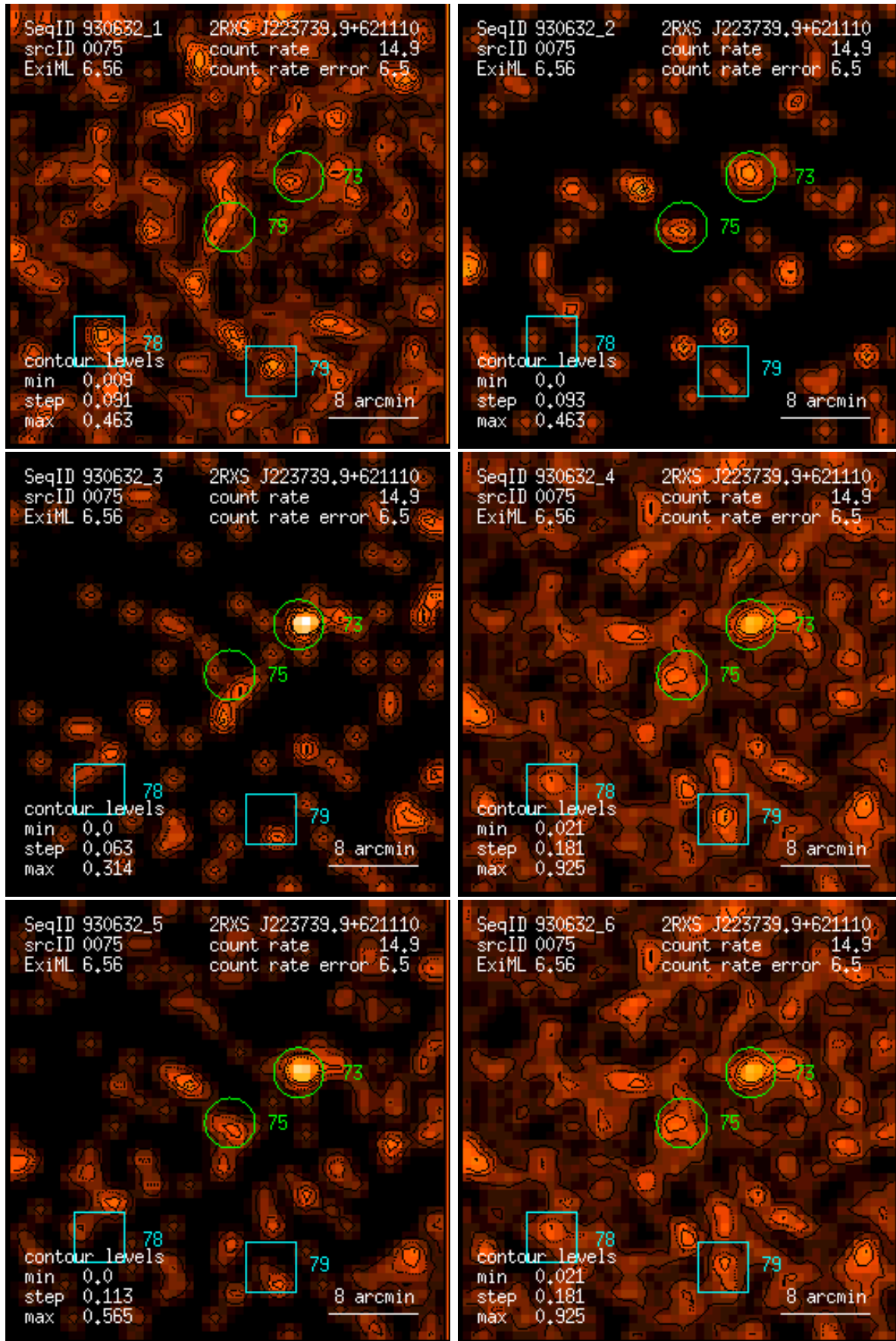
Figure 75: RASS 930632: detection 0075: band rate images, Gaussian filter: (1) PSPC channels 11 – 41, (2) 52 – 90, (3) 91 – 201, (4) 11 – 235, (5) 52 – 201, (6) 11 – 201. Broad band rates in counts/ks. Band rate contour levels in counts/ks/arcmin 2 .
