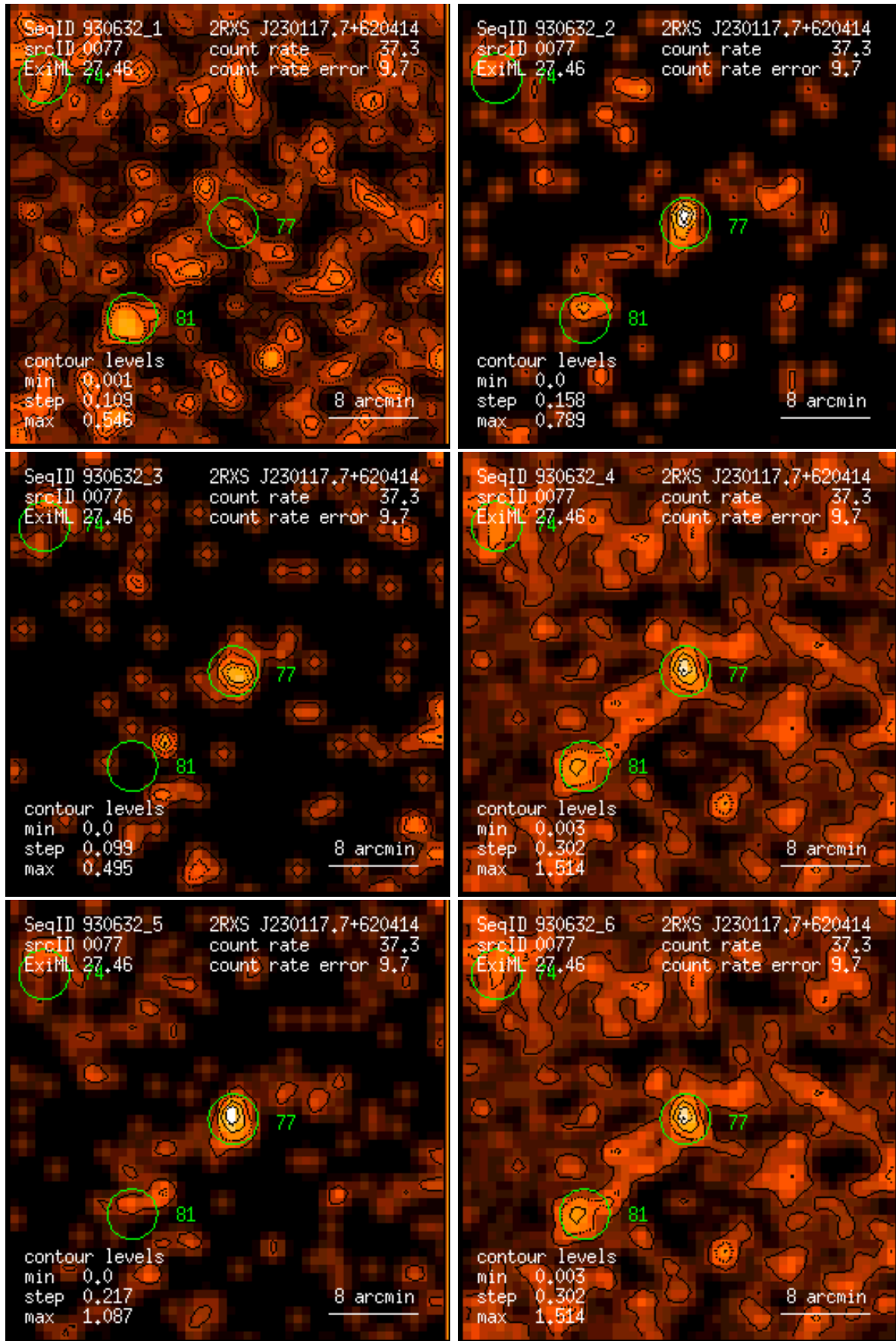
Figure 77: RASS 930632: detection 0077: band rate images, Gaussian filter: (1) PSPC channels 11 – 41, (2) 52 – 90, (3) 91 – 201, (4) 11 – 235, (5) 52 – 201, (6) 11 – 201. Broad band rates in counts/ks. Band rate contour levels in counts/ks/arcmin 2 .
