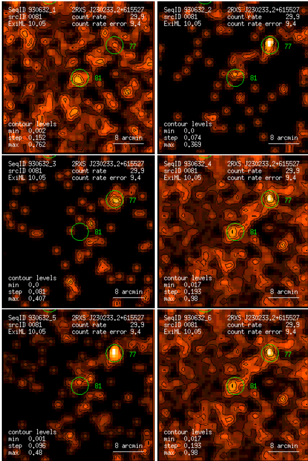
Figure 81: RASS 930632: detection 0081: band rate images, Gaussian filter: (1) PSPC channels 11 – 41, (2) 52 – 90, (3) 91 – 201, (4) 11 – 235, (5) 52 – 201, (6) 11 – 201. Broad band rates in counts/ks. Band rate contour levels in counts/ks/arcmin 2 .
