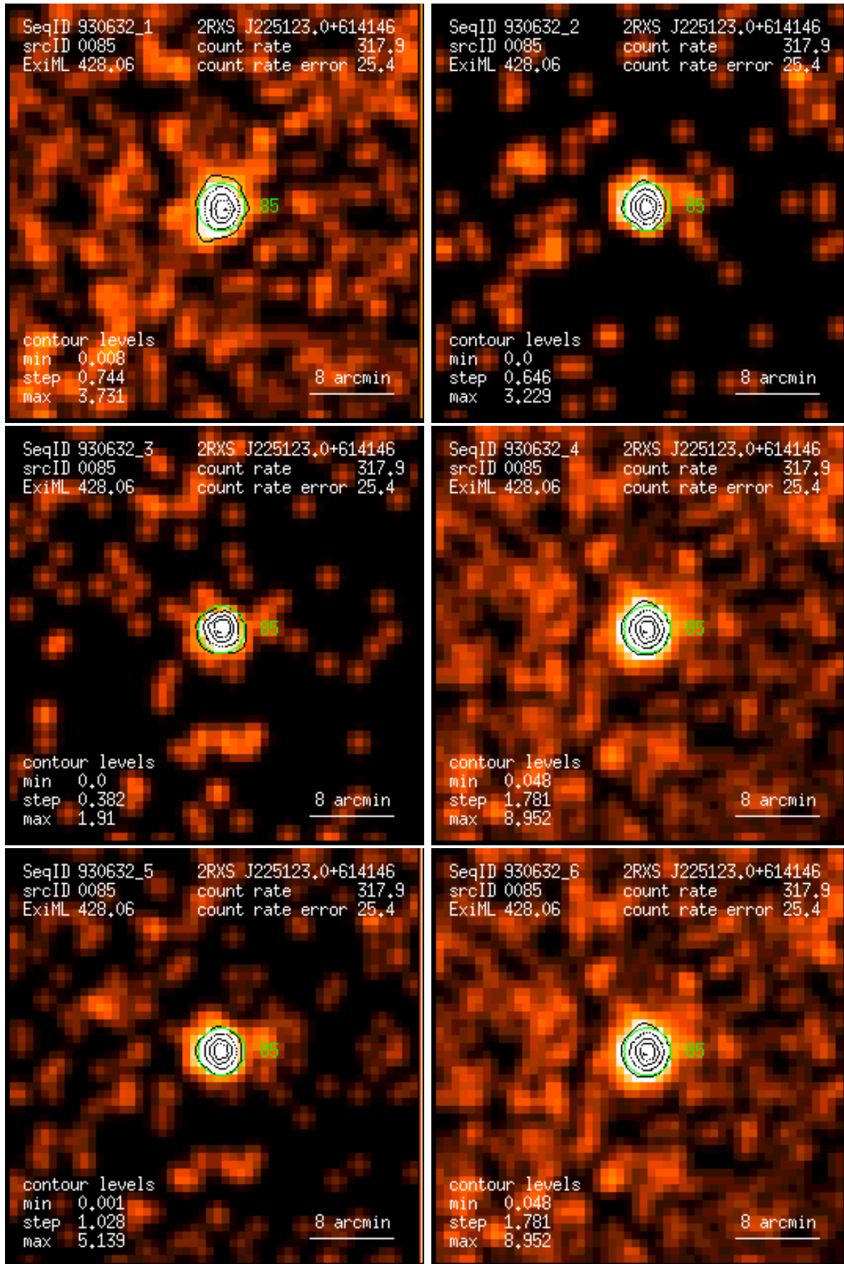
Figure 85: RASS 930632: detection 0085: band rate images, Gaussian filter: (1) PSPC channels 11 – 41, (2) 52 – 90, (3) 91 – 201, (4) 11 – 235, (5) 52 – 201, (6) 11 – 201. Broad band rates in counts/ks. Band rate contour levels in counts/ks/arcmin 2 .
