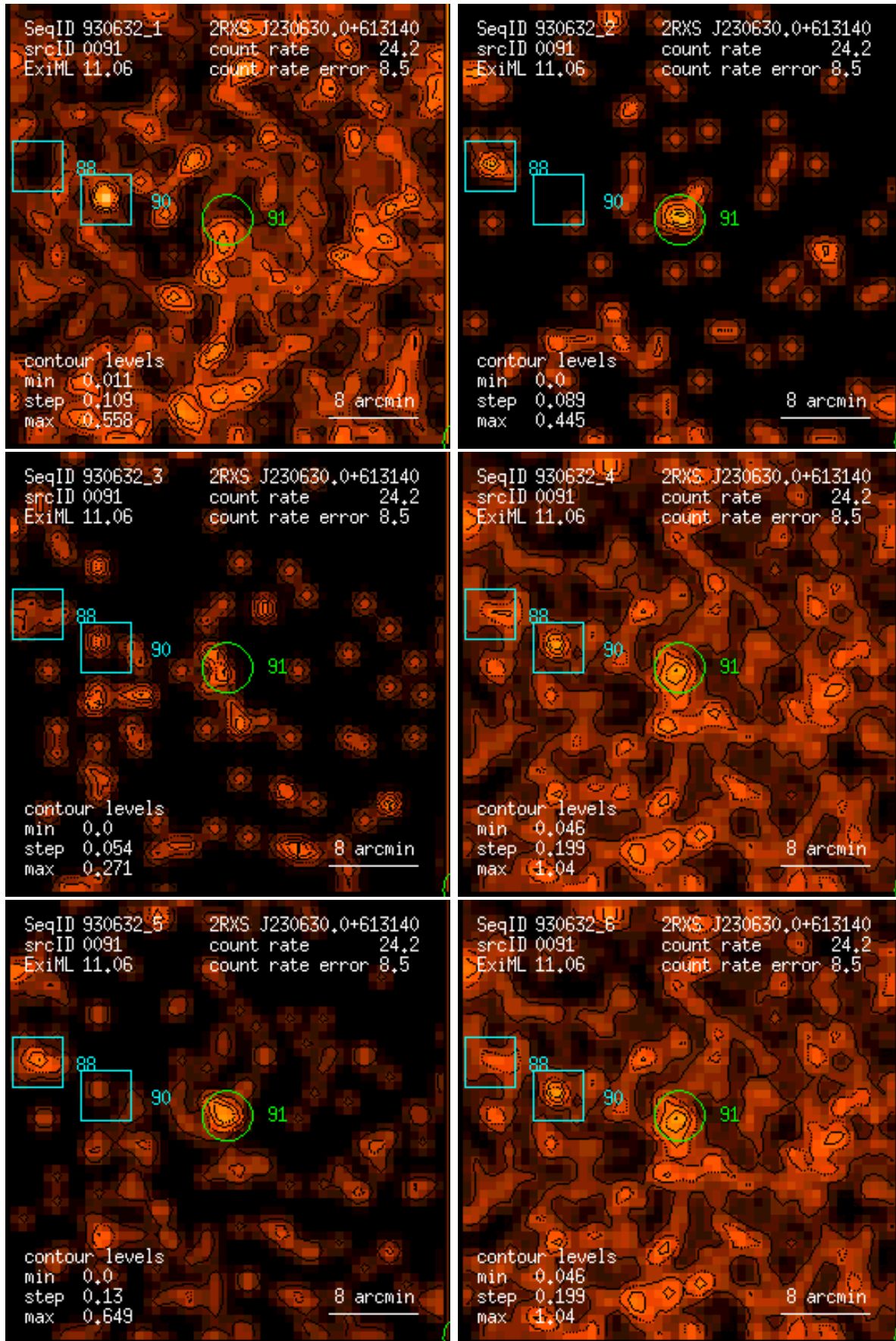
Figure 91: RASS 930632: detection 0091: band rate images, Gaussian filter: (1) PSPC channels 11 – 41, (2) 52 – 90, (3) 91 – 201, (4) 11 – 235, (5) 52 – 201, (6) 11 – 201. Broad band rates in counts/ks. Band rate contour levels in counts/ks/arcmin 2 .
