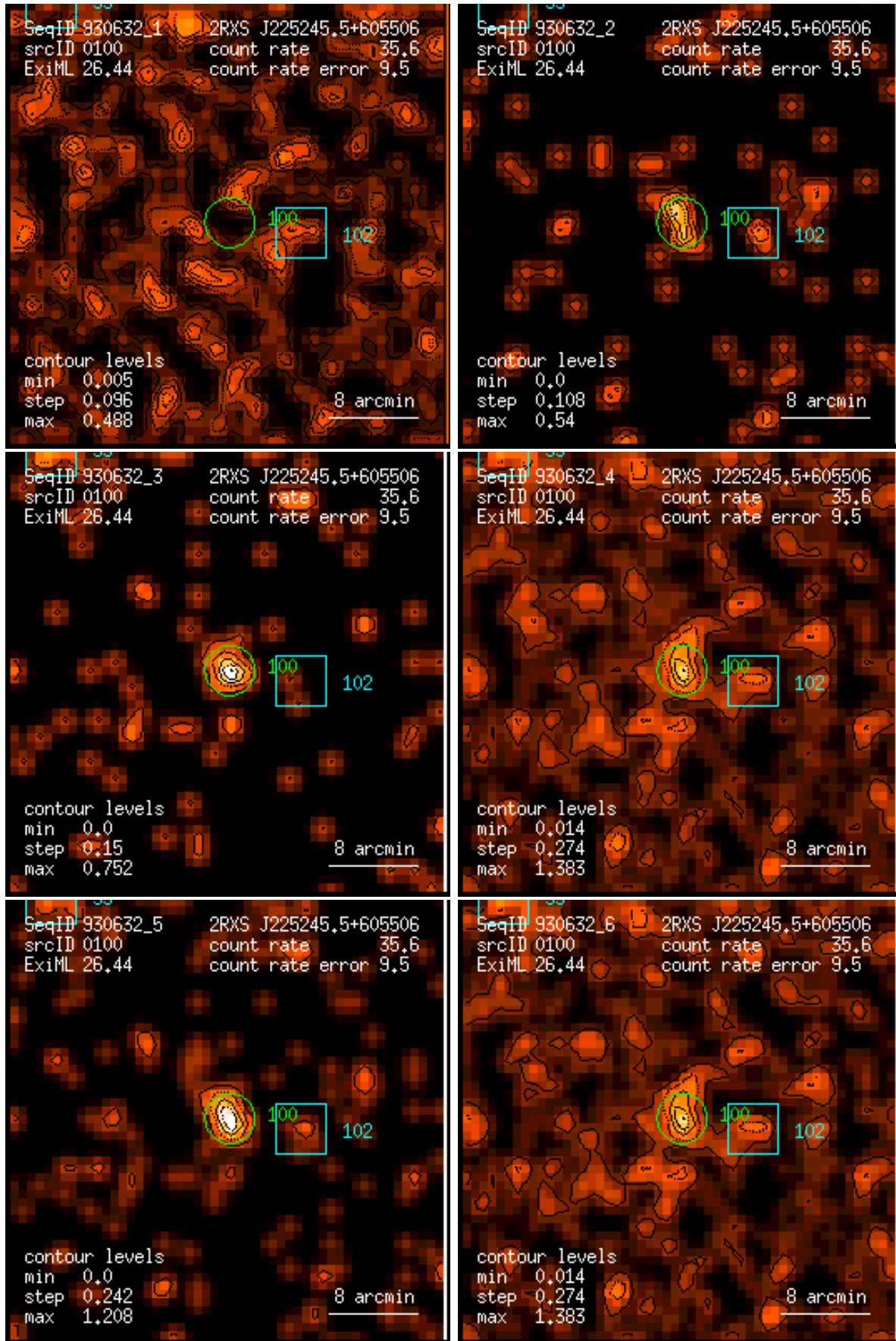
Figure 100: RASS 930632: detection 0100: band rate images, Gaussian filter: (1) PSPC channels 11 – 41, (2) 52 – 90, (3) 91 – 201, (4) 11 – 235, (5) 52 – 201, (6) 11 – 201. Broad band rates in counts/ks. Band rate contour levels in counts/ks/arcmin 2 .
