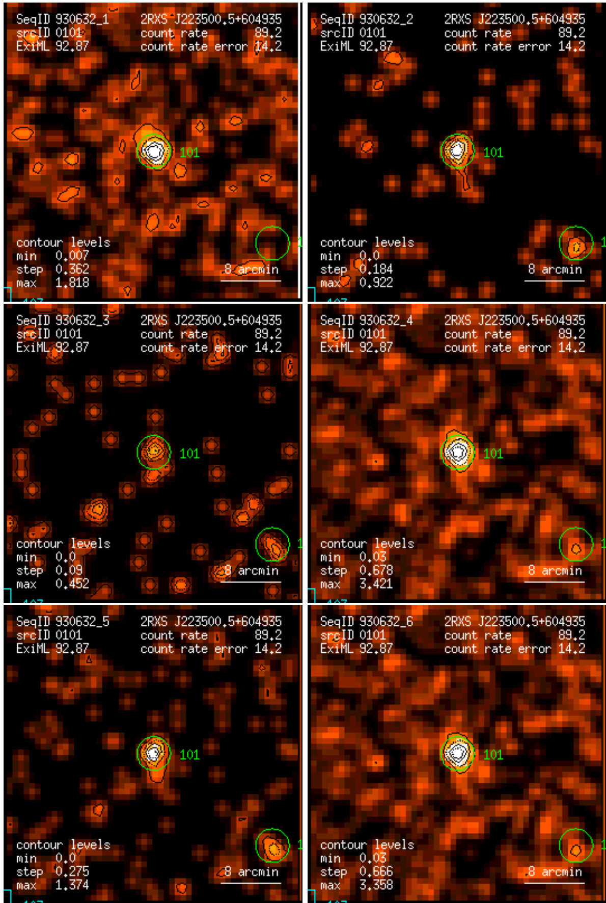
Figure 101: RASS 930632: detection 0101: band rate images, Gaussian filter: (1) PSPC channels 11 – 41, (2) 52 – 90, (3) 91 – 201, (4) 11 – 235, (5) 52 – 201, (6) 11 – 201. Broad band rates in counts/ks. Band rate contour levels in counts/ks/arcmin 2 .
