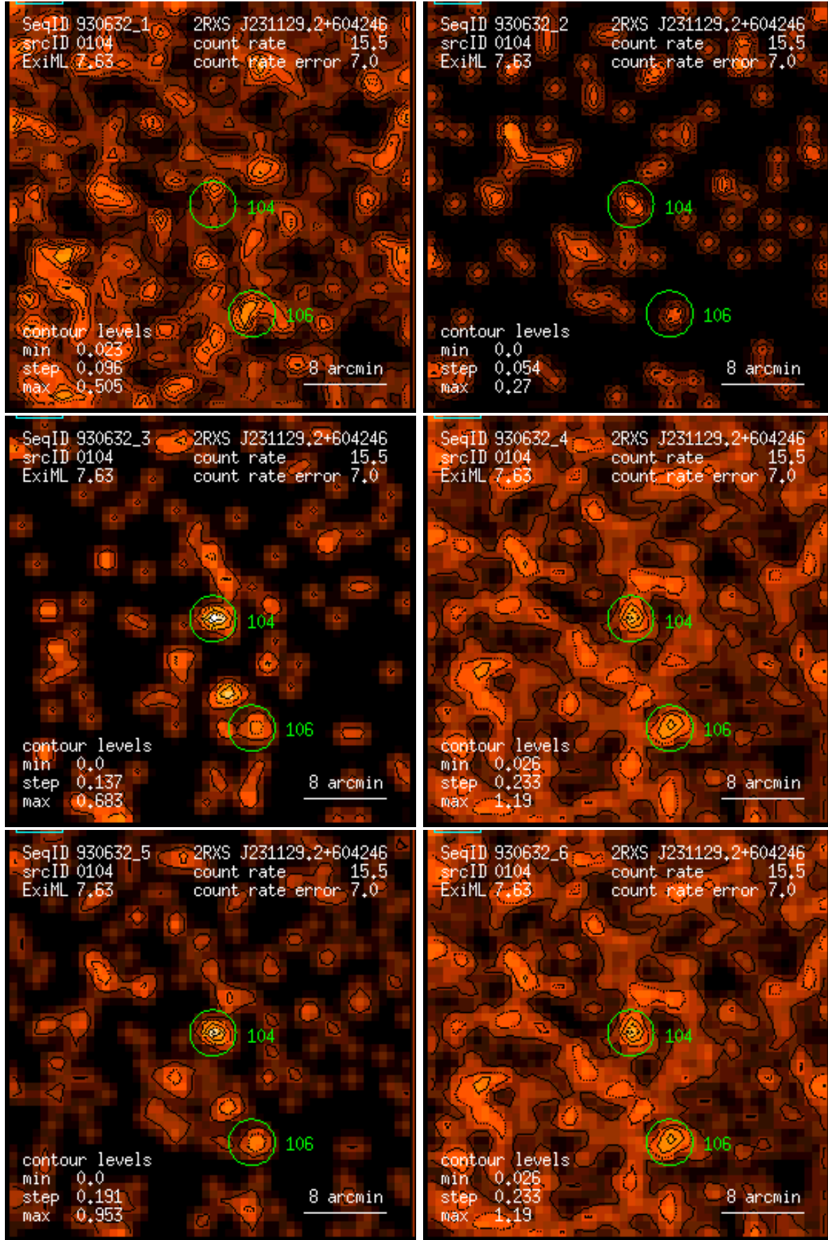
Figure 104: RASS 930632: detection 0104: band rate images, Gaussian filter: (1) PSPC channels 11 – 41, (2) 52 – 90, (3) 91 – 201, (4) 11 – 235, (5) 52 – 201, (6) 11 – 201. Broad band rates in counts/ks. Band rate contour levels in counts/ks/arcmin 2 .
