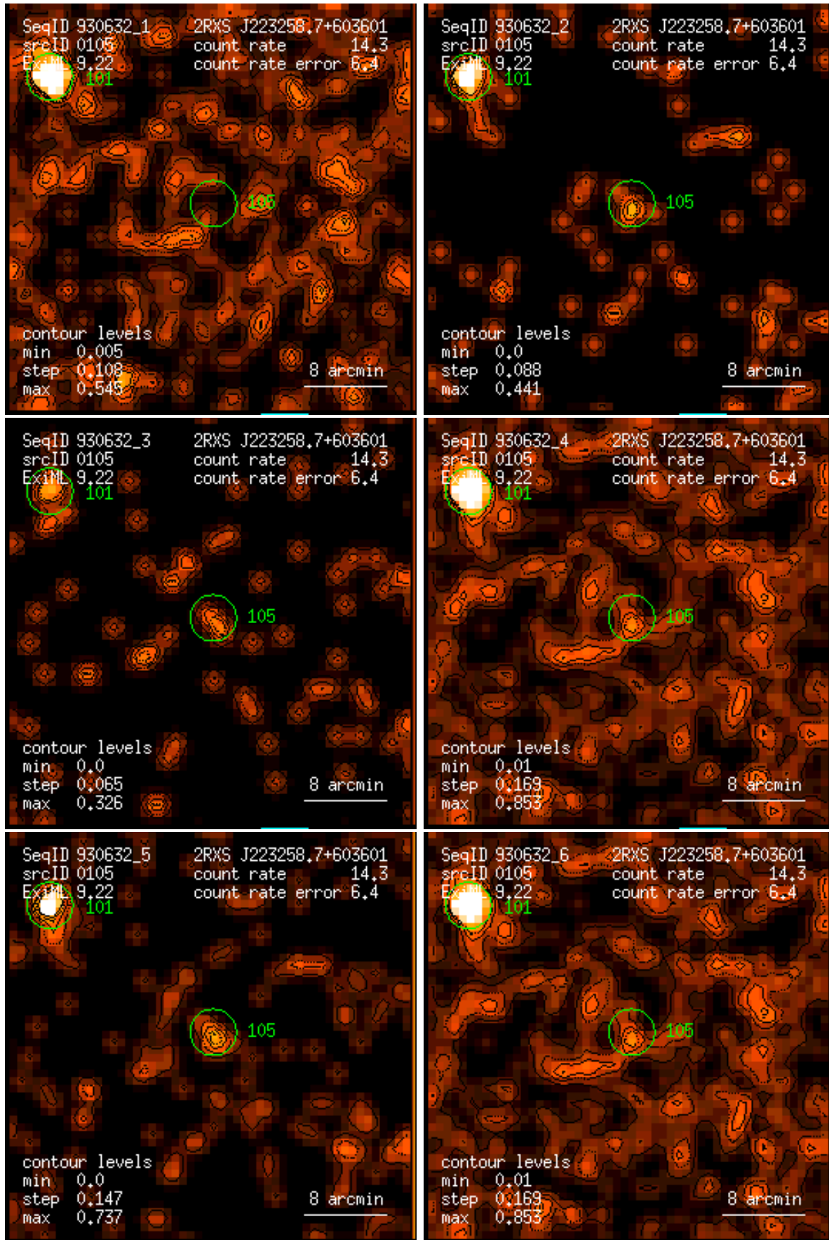
Figure 105: RASS 930632: detection 0105: band rate images, Gaussian filter: (1) PSPC channels 11 – 41, (2) 52 – 90, (3) 91 – 201, (4) 11 – 235, (5) 52 – 201, (6) 11 – 201. Broad band rates in counts/ks. Band rate contour levels in counts/ks/arcmin 2 .
