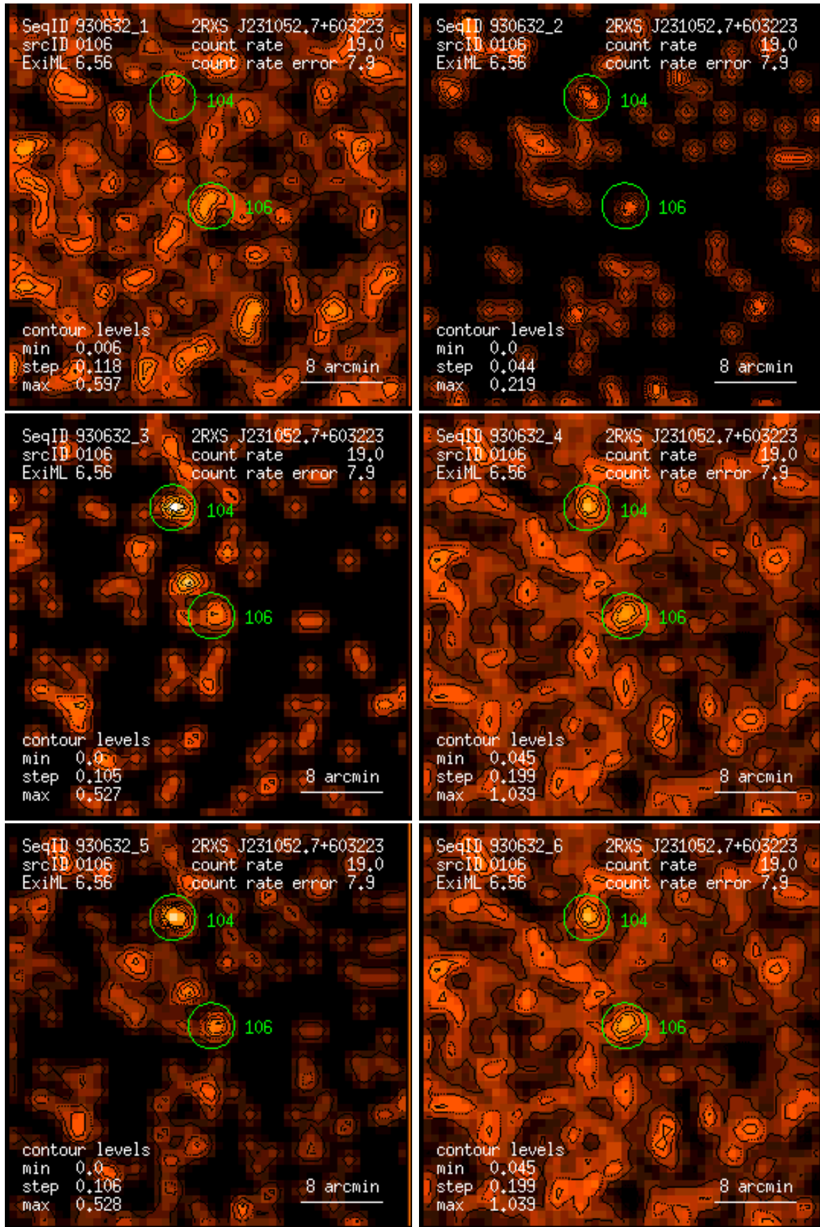
Figure 106: RASS 930632: detection 0106: band rate images, Gaussian filter: (1) PSPC channels 11 – 41, (2) 52 – 90, (3) 91 – 201, (4) 11 – 235, (5) 52 – 201, (6) 11 – 201. Broad band rates in counts/ks. Band rate contour levels in counts/ks/arcmin 2 .
