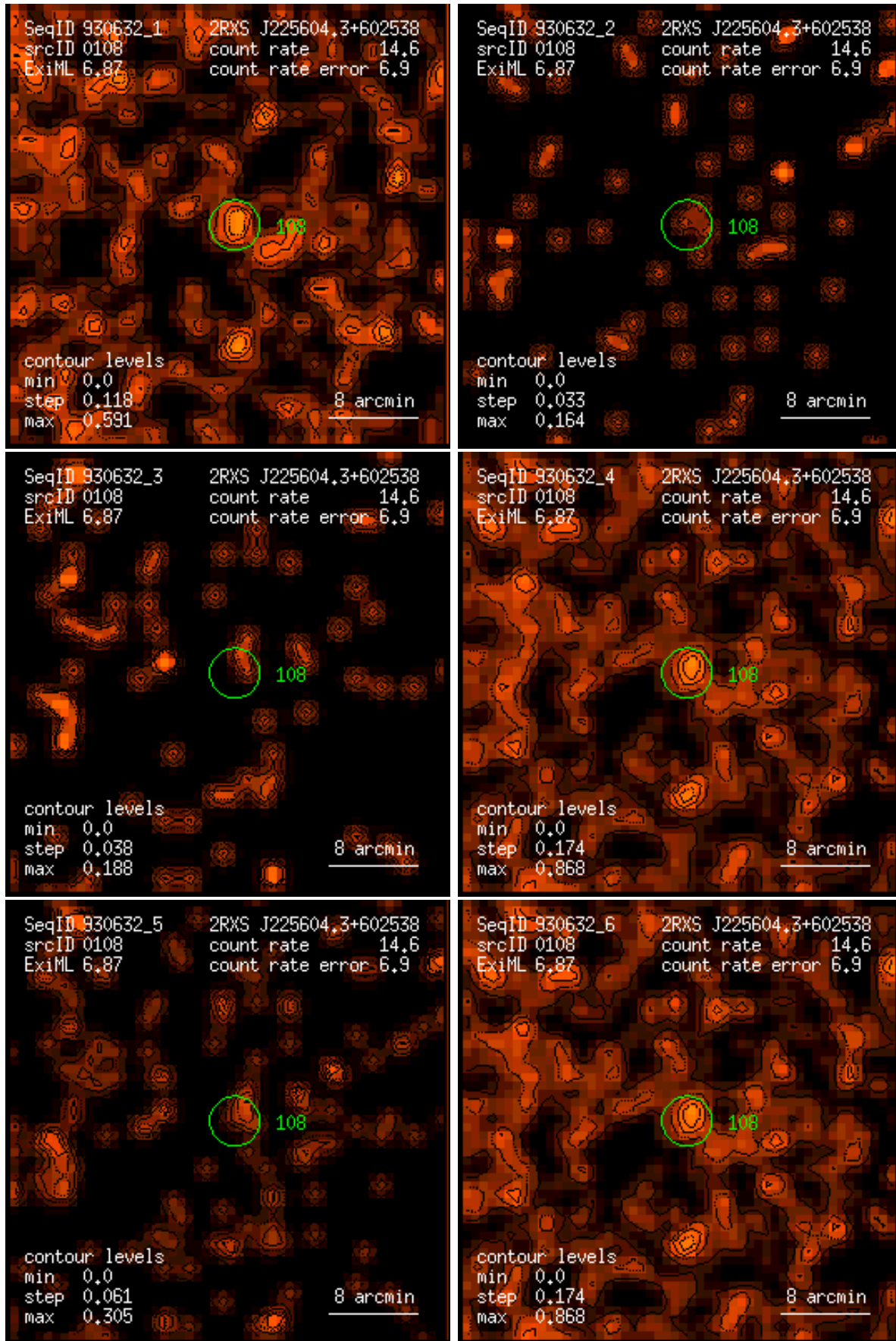
Figure 108: RASS 930632: detection 0108: band rate images, Gaussian filter: (1) PSPC channels 11 – 41, (2) 52 – 90, (3) 91 – 201, (4) 11 – 235, (5) 52 – 201, (6) 11 – 201. Broad band rates in counts/ks. Band rate contour levels in counts/ks/arcmin 2 .
