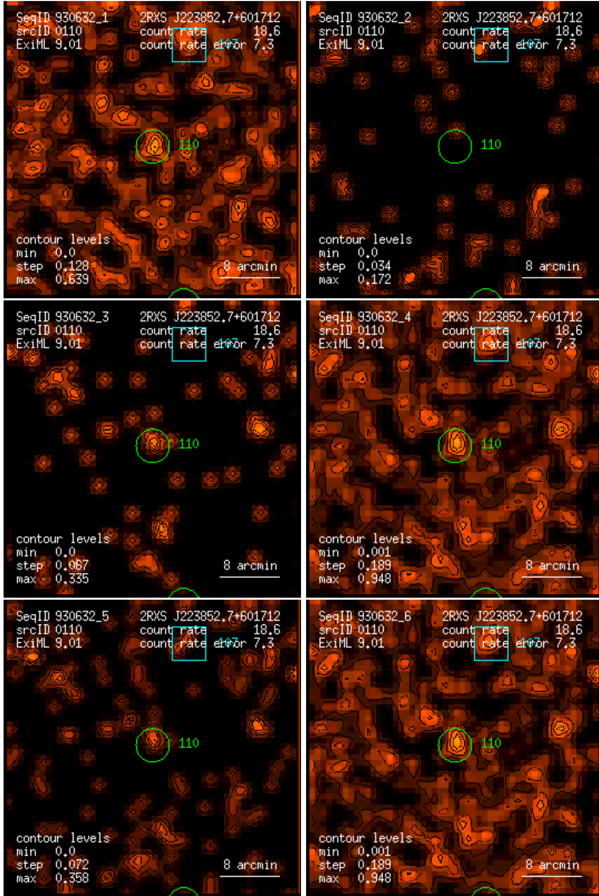
Figure 110: RASS 930632: detection 0110: band rate images, Gaussian filter: (1) PSPC channels 11 – 41, (2) 52 – 90, (3) 91 – 201, (4) 11 – 235, (5) 52 – 201, (6) 11 – 201. Broad band rates in counts/ks. Band rate contour levels in counts/ks/arcmin 2 .
