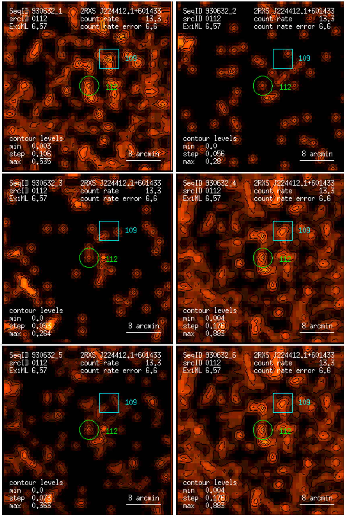
Figure 112: RASS 930632: detection 0112: band rate images, Gaussian filter: (1) PSPC channels 11 – 41, (2) 52 – 90, (3) 91 – 201, (4) 11 – 235, (5) 52 – 201, (6) 11 – 201. Broad band rates in counts/ks. Band rate contour levels in counts/ks/arcmin 2 .
