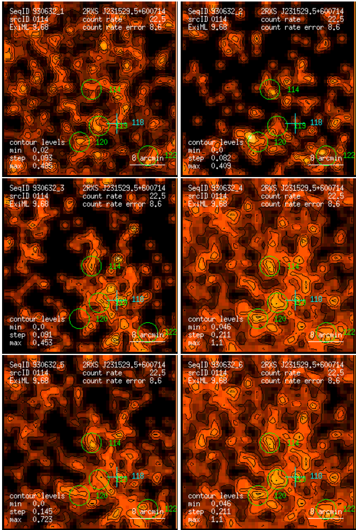
Figure 114: RASS 930632: detection 0114: band rate images, Gaussian filter: (1) PSPC channels 11 – 41, (2) 52 – 90, (3) 91 – 201, (4) 11 – 235, (5) 52 – 201, (6) 11 – 201. Broad band rates in counts/ks. Band rate contour levels in counts/ks/arcmin 2 .
