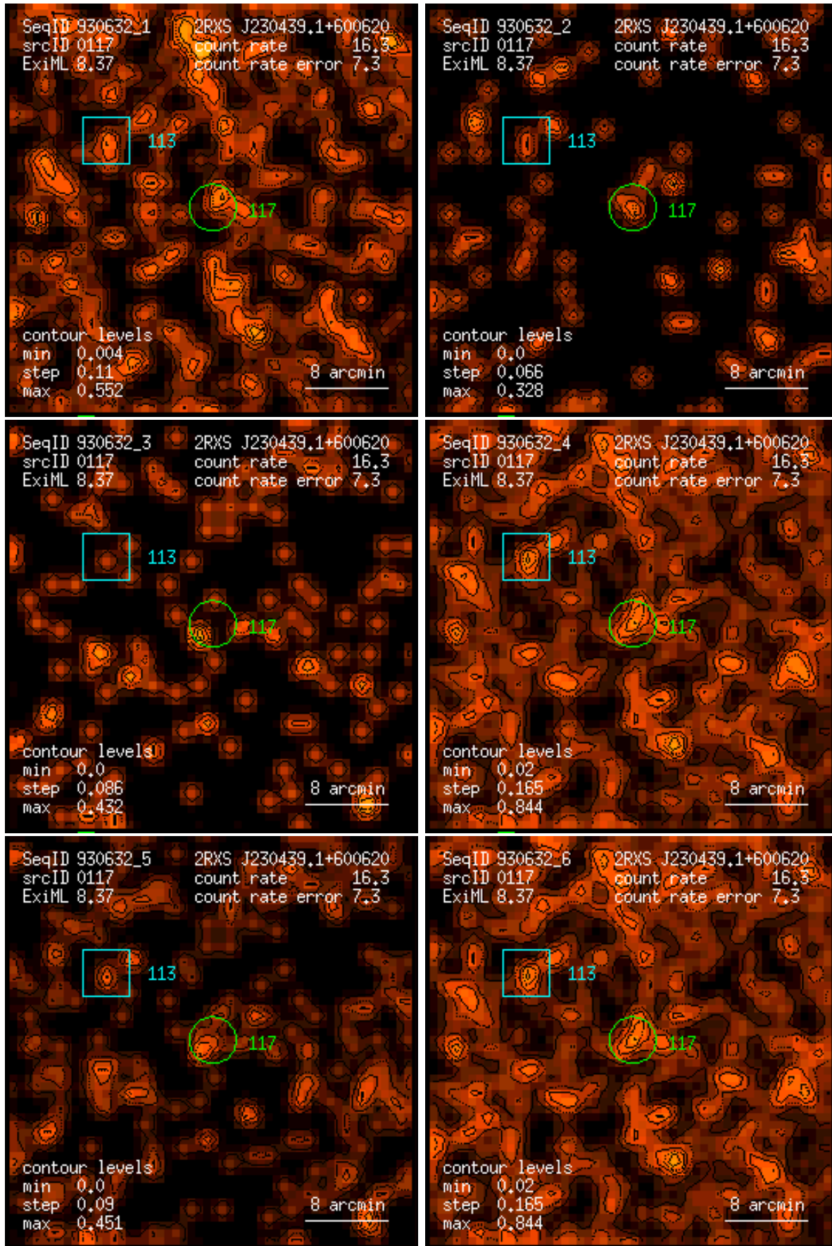
Figure 117: RASS 930632: detection 0117: band rate images, Gaussian filter: (1) PSPC channels 11 – 41, (2) 52 – 90, (3) 91 – 201, (4) 11 – 235, (5) 52 – 201, (6) 11 – 201. Broad band rates in counts/ks. Band rate contour levels in counts/ks/arcmin 2 .
