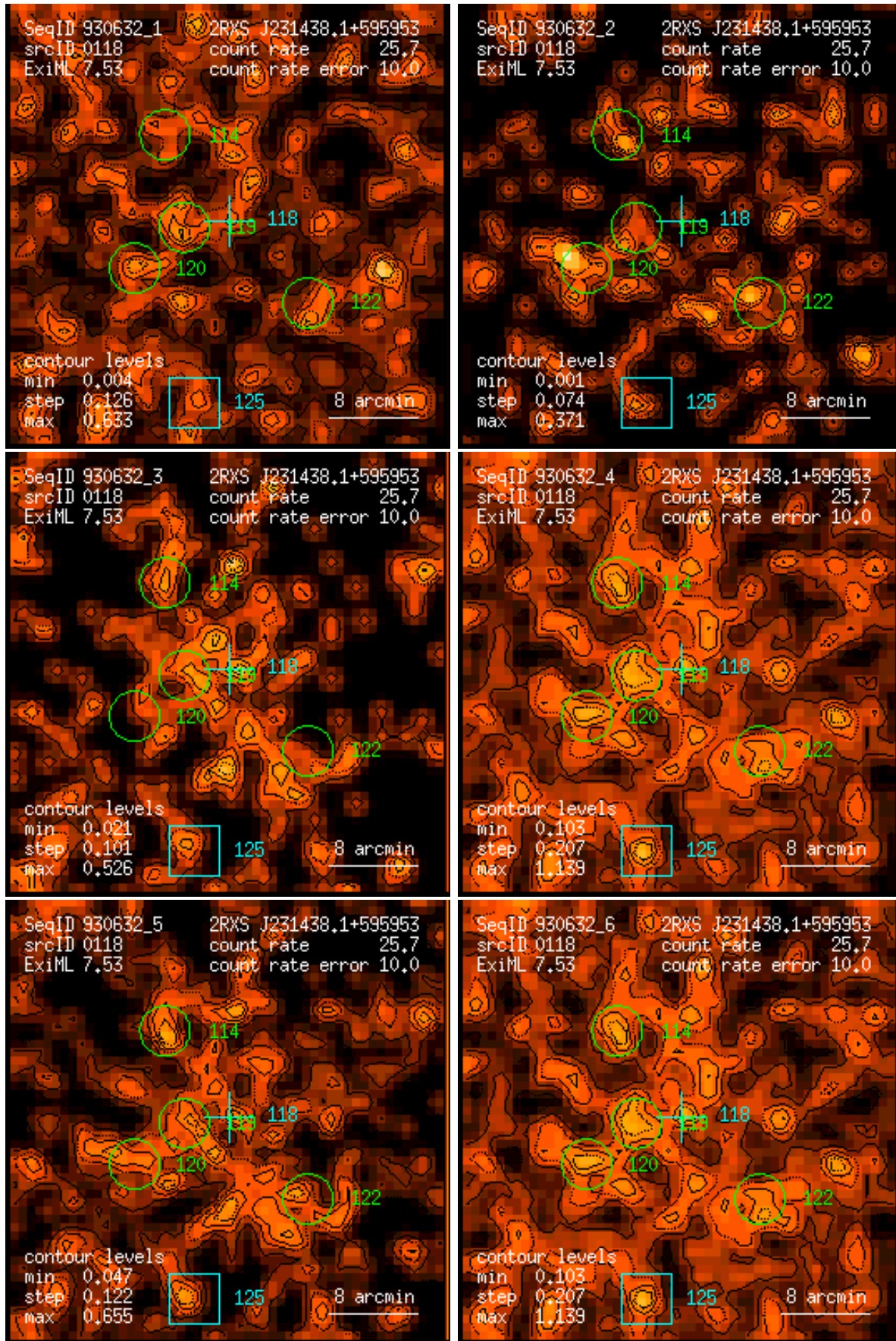
Figure 118: RASS 930632: detection 0118: band rate images, Gaussian filter: (1) PSPC channels 11 – 41, (2) 52 – 90, (3) 91 – 201, (4) 11 – 235, (5) 52 – 201, (6) 11 – 201. Broad band rates in counts/ks. Band rate contour levels in counts/ks/arcmin 2 .
