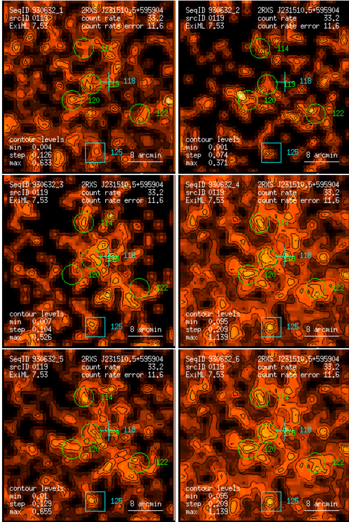
Figure 119: RASS 930632: detection 0119: band rate images, Gaussian filter: (1) PSPC channels 11 – 41, (2) 52 – 90, (3) 91 – 201, (4) 11 – 235, (5) 52 – 201, (6) 11 – 201. Broad band rates in counts/ks. Band rate contour levels in counts/ks/arcmin 2 .
