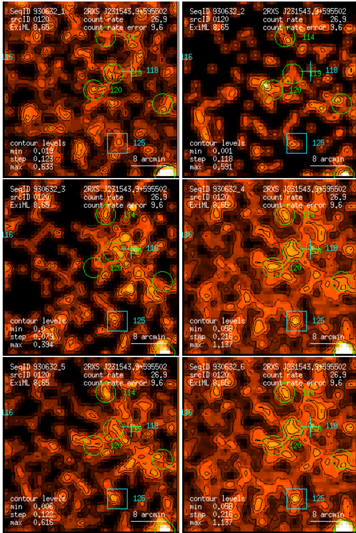
Figure 120: RASS 930632: detection 0120: band rate images, Gaussian filter: (1) PSPC channels 11 – 41, (2) 52 – 90, (3) 91 – 201, (4) 11 – 235, (5) 52 – 201, (6) 11 – 201. Broad band rates in counts/ks. Band rate contour levels in counts/ks/arcmin 2 .
