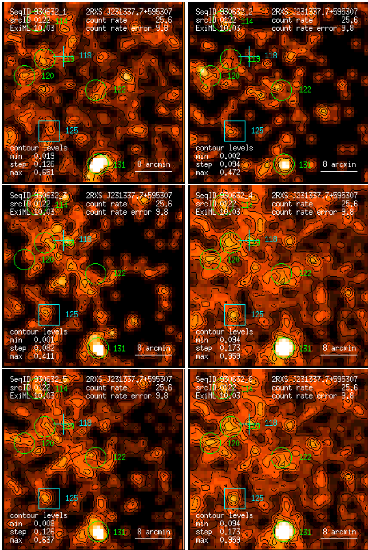
Figure 122: RASS 930632: detection 0122: band rate images, Gaussian filter: (1) PSPC channels 11 – 41, (2) 52 – 90, (3) 91 – 201, (4) 11 – 235, (5) 52 – 201, (6) 11 – 201. Broad band rates in counts/ks. Band rate contour levels in counts/ks/arcmin 2 .
