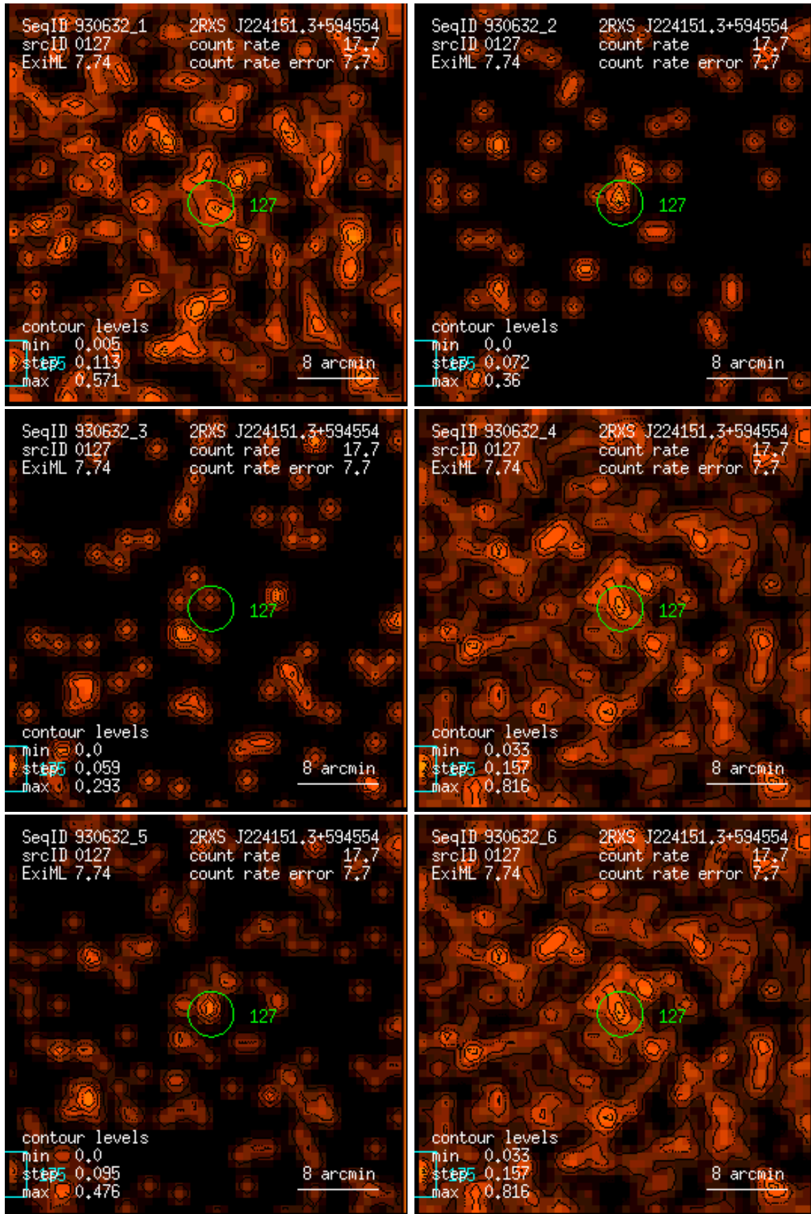
Figure 127: RASS 930632: detection 0127: band rate images, Gaussian filter: (1) PSPC channels 11 – 41, (2) 52 – 90, (3) 91 – 201, (4) 11 – 235, (5) 52 – 201, (6) 11 – 201. Broad band rates in counts/ks. Band rate contour levels in counts/ks/arcmin 2 .
