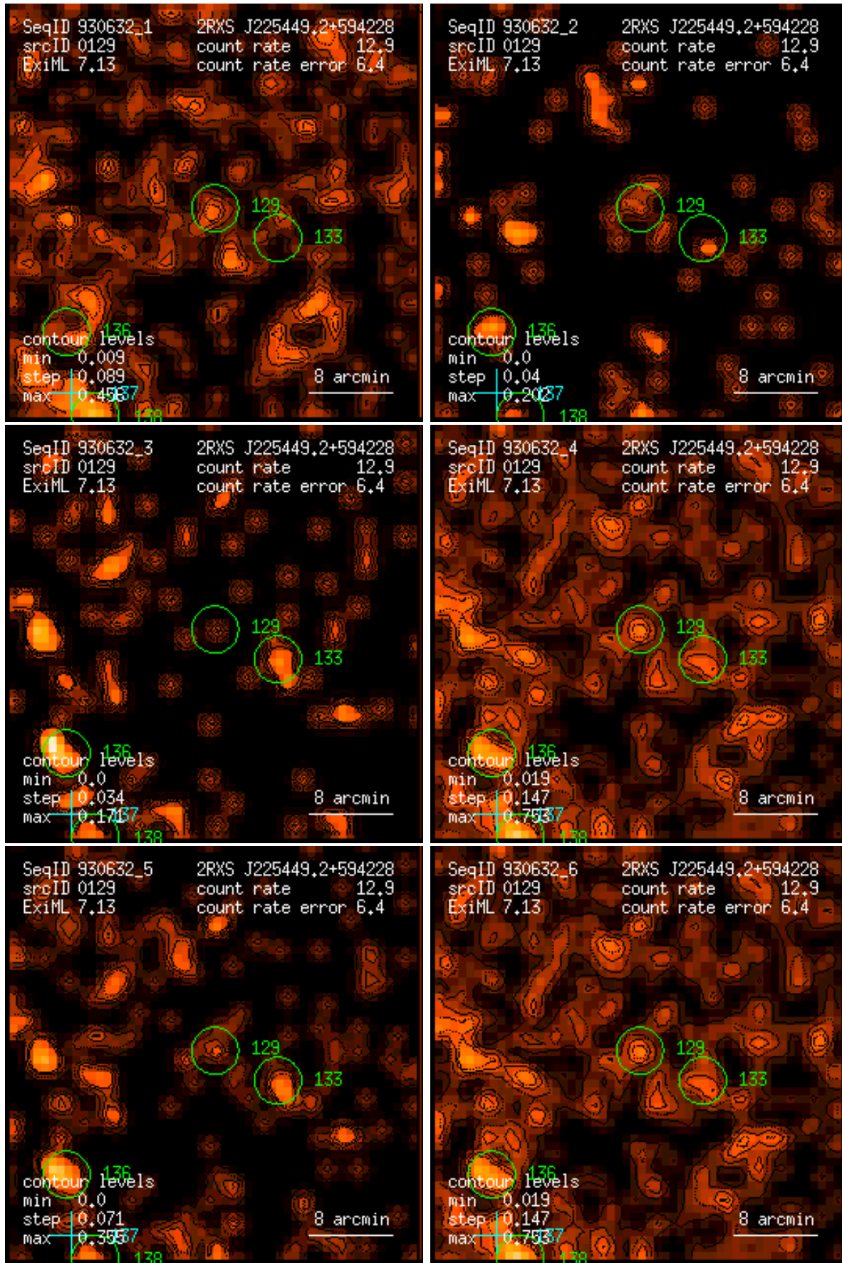
Figure 129: RASS 930632: detection 0129: band rate images, Gaussian filter: (1) PSPC channels 11 – 41, (2) 52 – 90, (3) 91 – 201, (4) 11 – 235, (5) 52 – 201, (6) 11 – 201. Broad band rates in counts/ks. Band rate contour levels in counts/ks/arcmin 2 .
