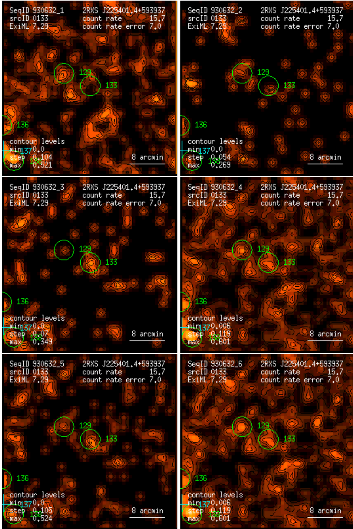
Figure 133: RASS 930632: detection 0133: band rate images, Gaussian filter: (1) PSPC channels 11 – 41, (2) 52 – 90, (3) 91 – 201, (4) 11 – 235, (5) 52 – 201, (6) 11 – 201. Broad band rates in counts/ks. Band rate contour levels in counts/ks/arcmin 2 .
