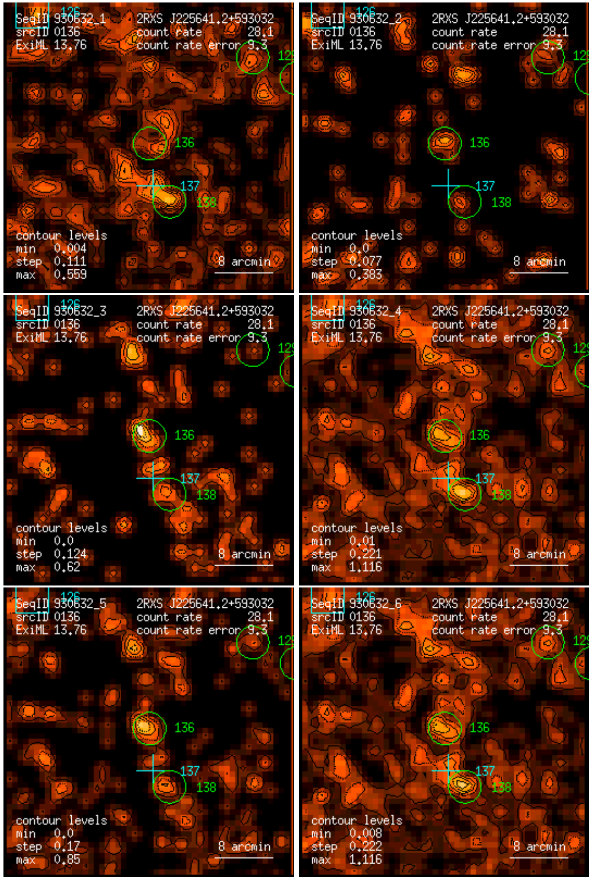
Figure 136: RASS 930632: detection 0136: band rate images, Gaussian filter: (1) PSPC channels 11 – 41, (2) 52 – 90, (3) 91 – 201, (4) 11 – 235, (5) 52 – 201, (6) 11 – 201. Broad band rates in counts/ks. Band rate contour levels in counts/ks/arcmin 2 .
