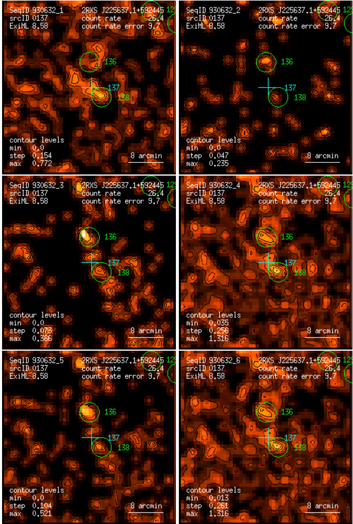
Figure 137: RASS 930632: detection 0137: band rate images, Gaussian filter: (1) PSPC channels 11 – 41, (2) 52 – 90, (3) 91 – 201, (4) 11 – 235, (5) 52 – 201, (6) 11 – 201. Broad band rates in counts/ks. Band rate contour levels in counts/ks/arcmin 2 .
