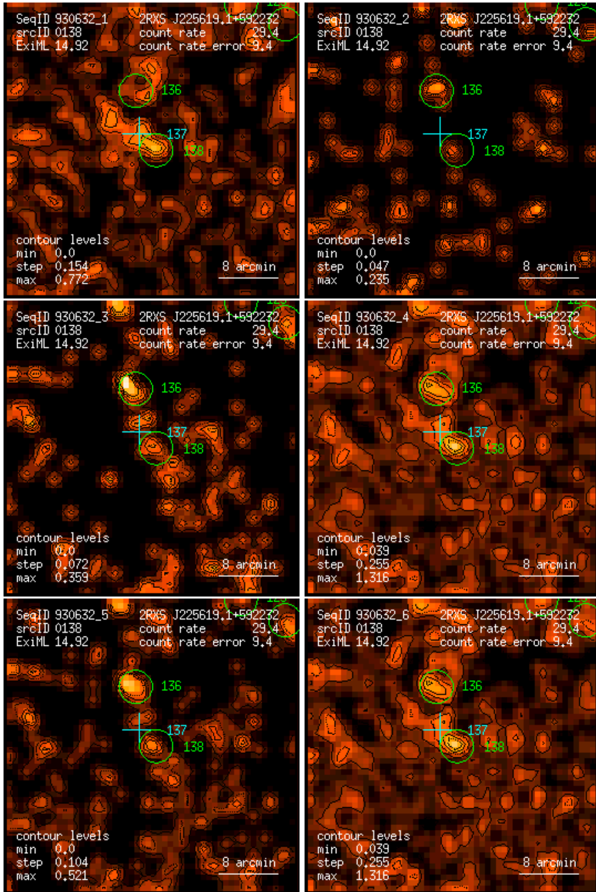
Figure 138: RASS 930632: detection 0138: band rate images, Gaussian filter: (1) PSPC channels 11 – 41, (2) 52 – 90, (3) 91 – 201, (4) 11 – 235, (5) 52 – 201, (6) 11 – 201. Broad band rates in counts/ks. Band rate contour levels in counts/ks/arcmin 2 .
