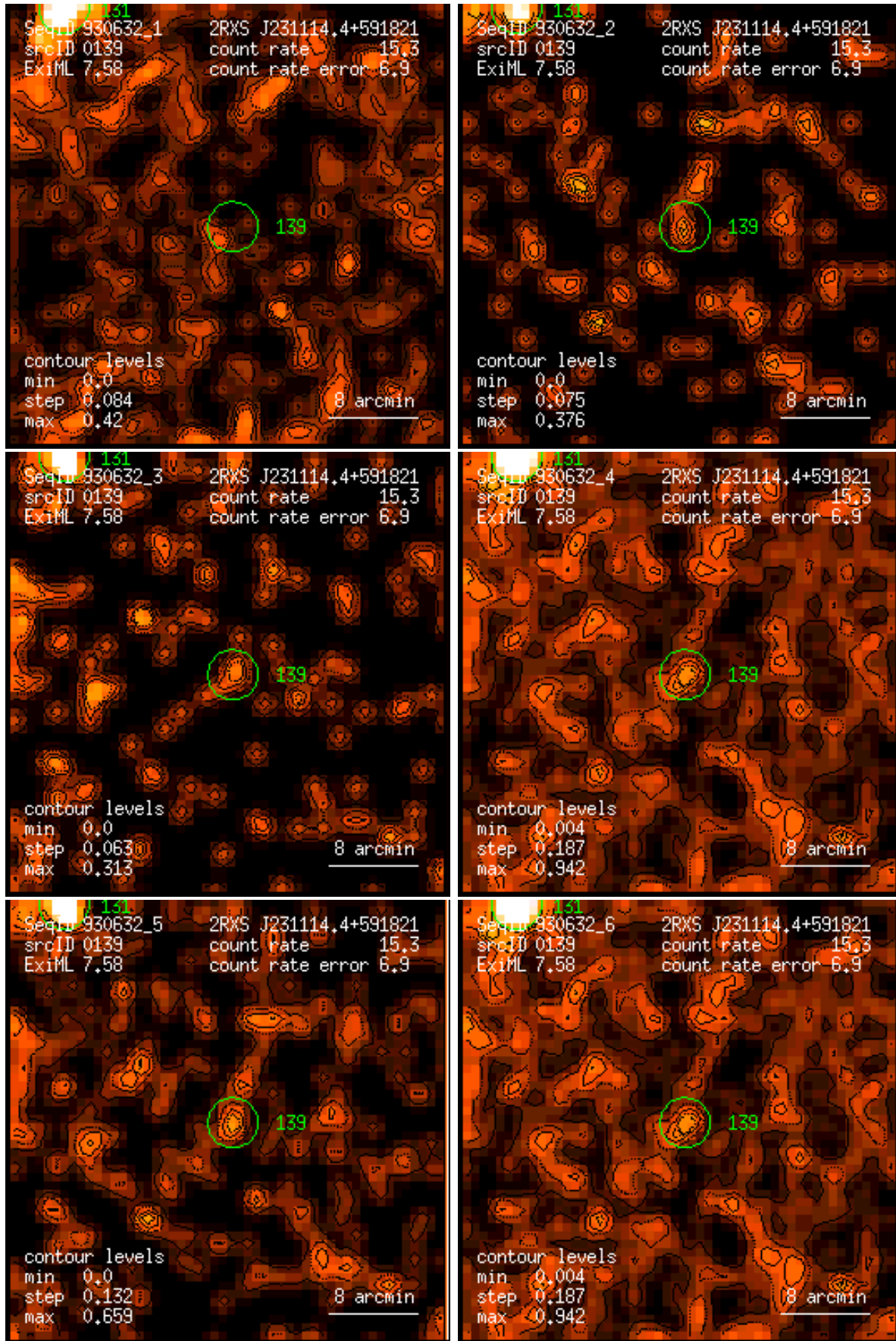
Figure 139: RASS 930632: detection 0139: band rate images, Gaussian filter: (1) PSPC channels 11 – 41, (2) 52 – 90, (3) 91 – 201, (4) 11 – 235, (5) 52 – 201, (6) 11 – 201. Broad band rates in counts/ks. Band rate contour levels in counts/ks/arcmin 2 .
