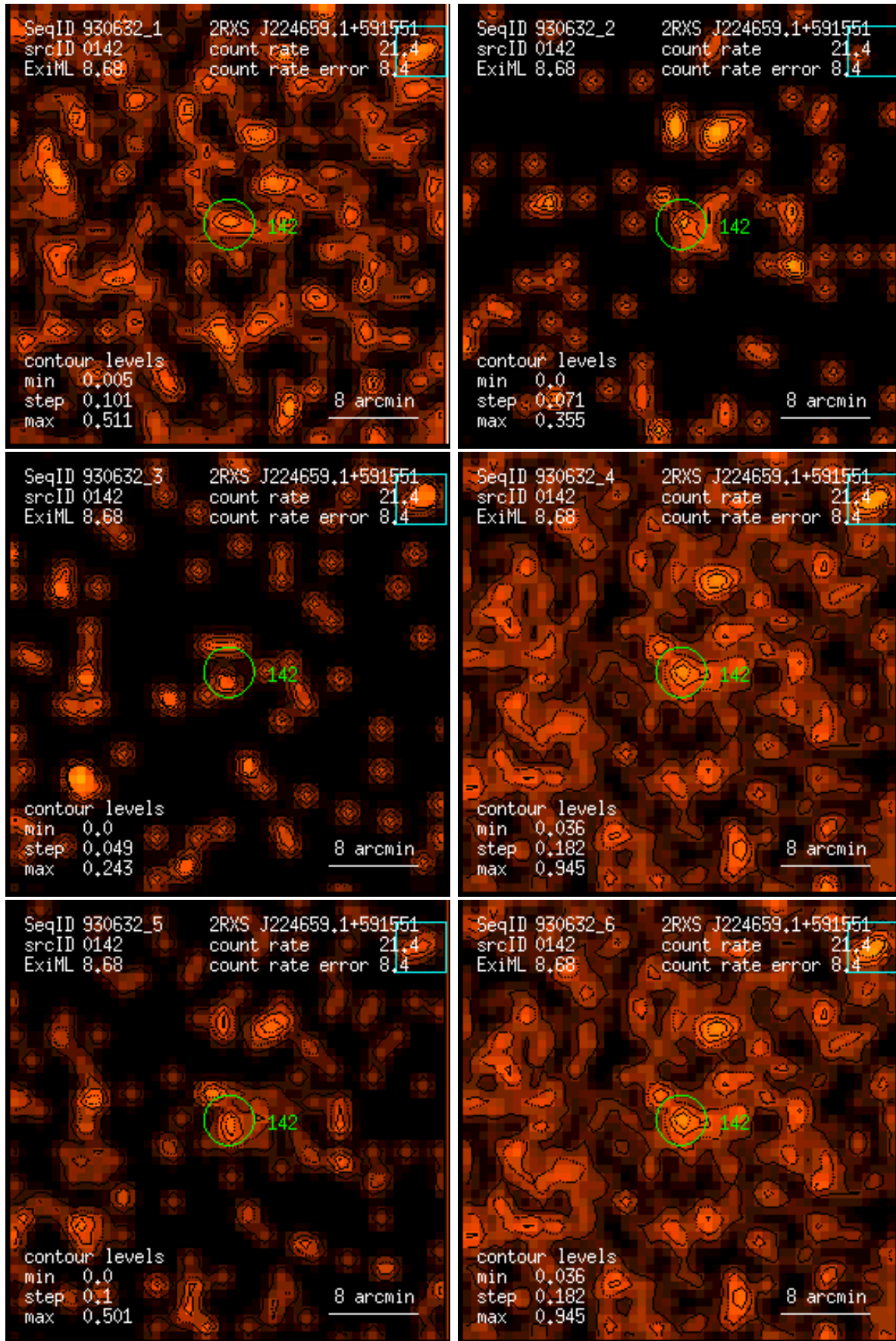
Figure 142: RASS 930632: detection 0142: band rate images, Gaussian filter: (1) PSPC channels 11 – 41, (2) 52 – 90, (3) 91 – 201, (4) 11 – 235, (5) 52 – 201, (6) 11 – 201. Broad band rates in counts/ks. Band rate contour levels in counts/ks/arcmin 2 .
