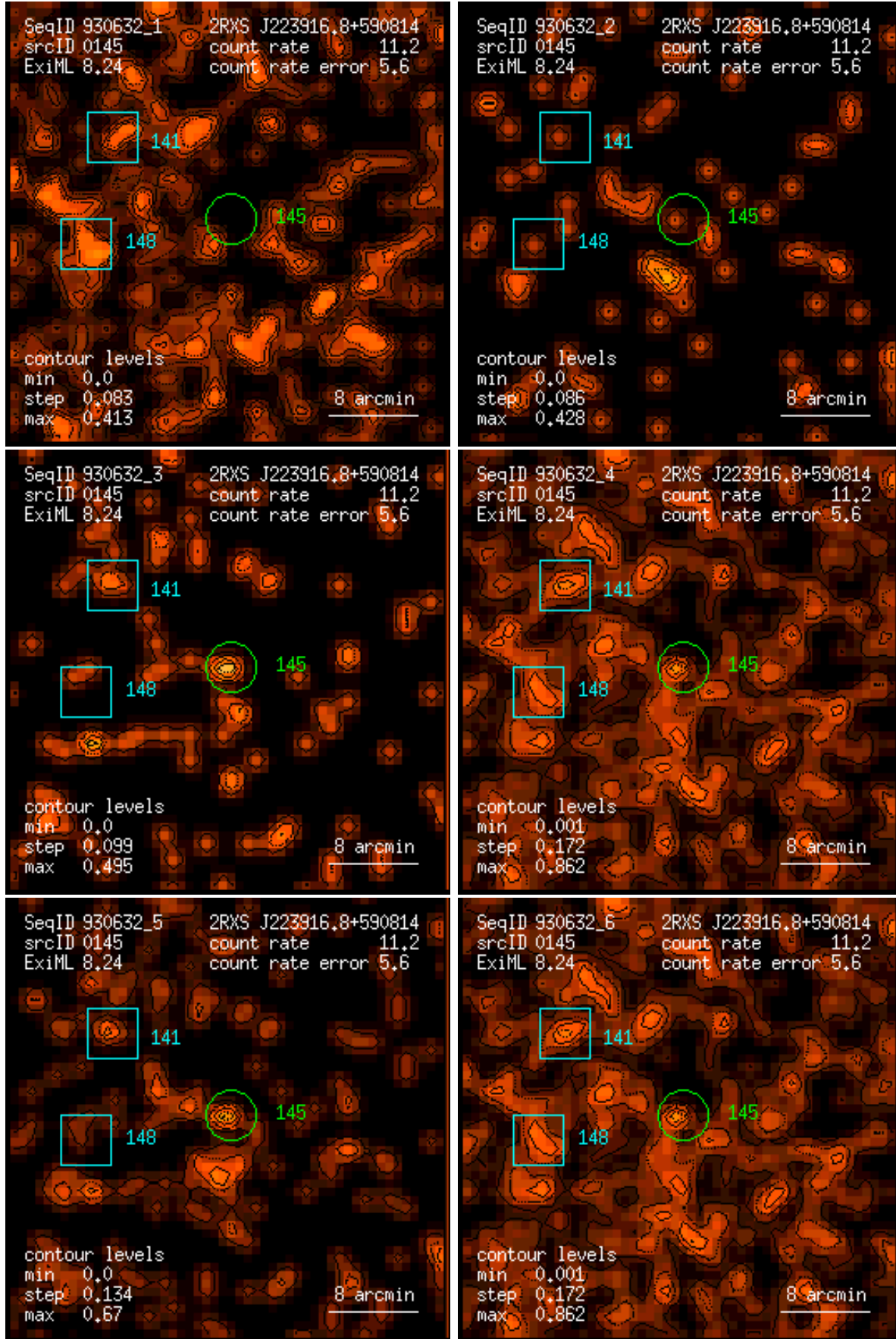
Figure 145: RASS 930632: detection 0145: band rate images, Gaussian filter: (1) PSPC channels 11 – 41, (2) 52 – 90, (3) 91 – 201, (4) 11 – 235, (5) 52 – 201, (6) 11 – 201. Broad band rates in counts/ks. Band rate contour levels in counts/ks/arcmin 2 .
