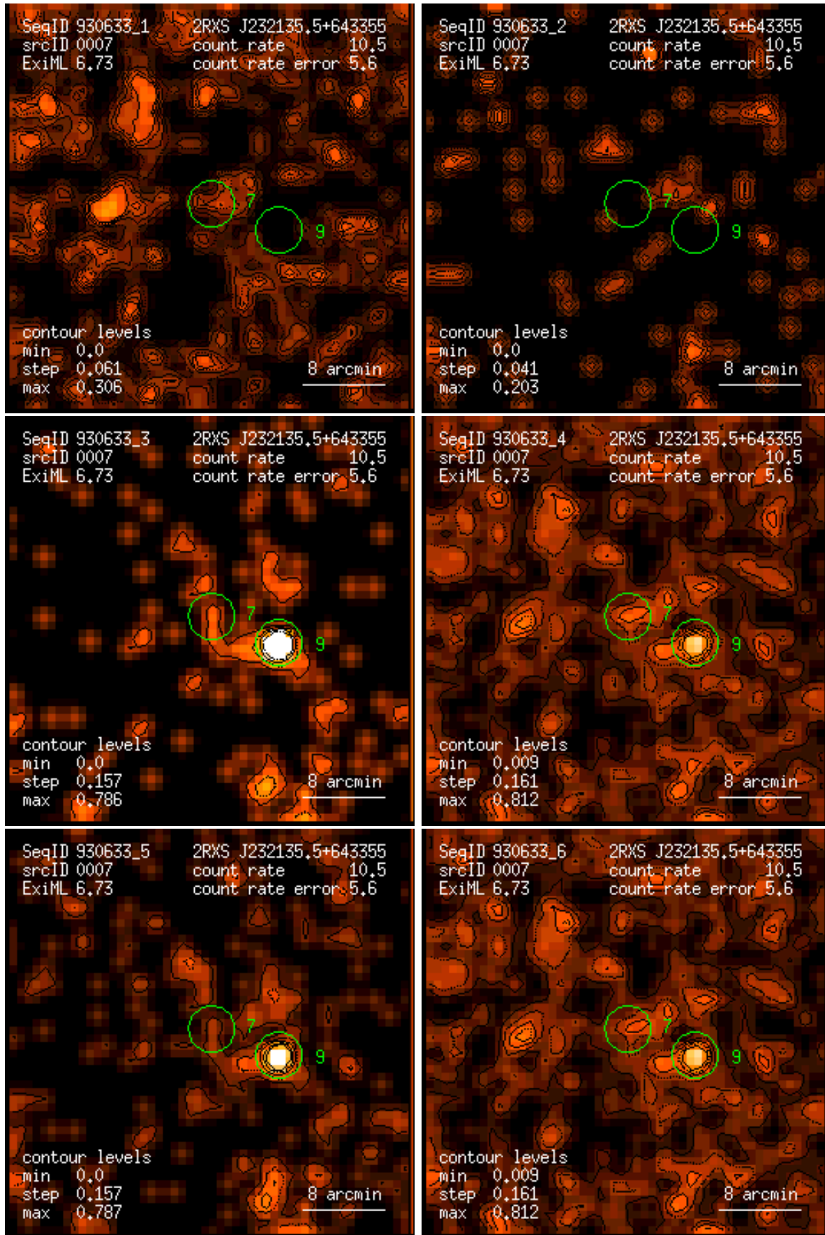
Figure 7: RASS 930633: detection 0007: band rate images, Gaussian filter: (1) PSPC channels 11 – 41, (2) 52 – 90, (3) 91 – 201, (4) 11 – 235, (5) 52 – 201, (6) 11 – 201. Broad band rates in counts/ks. Band rate contour levels in counts/ks/arcmin 2 .
