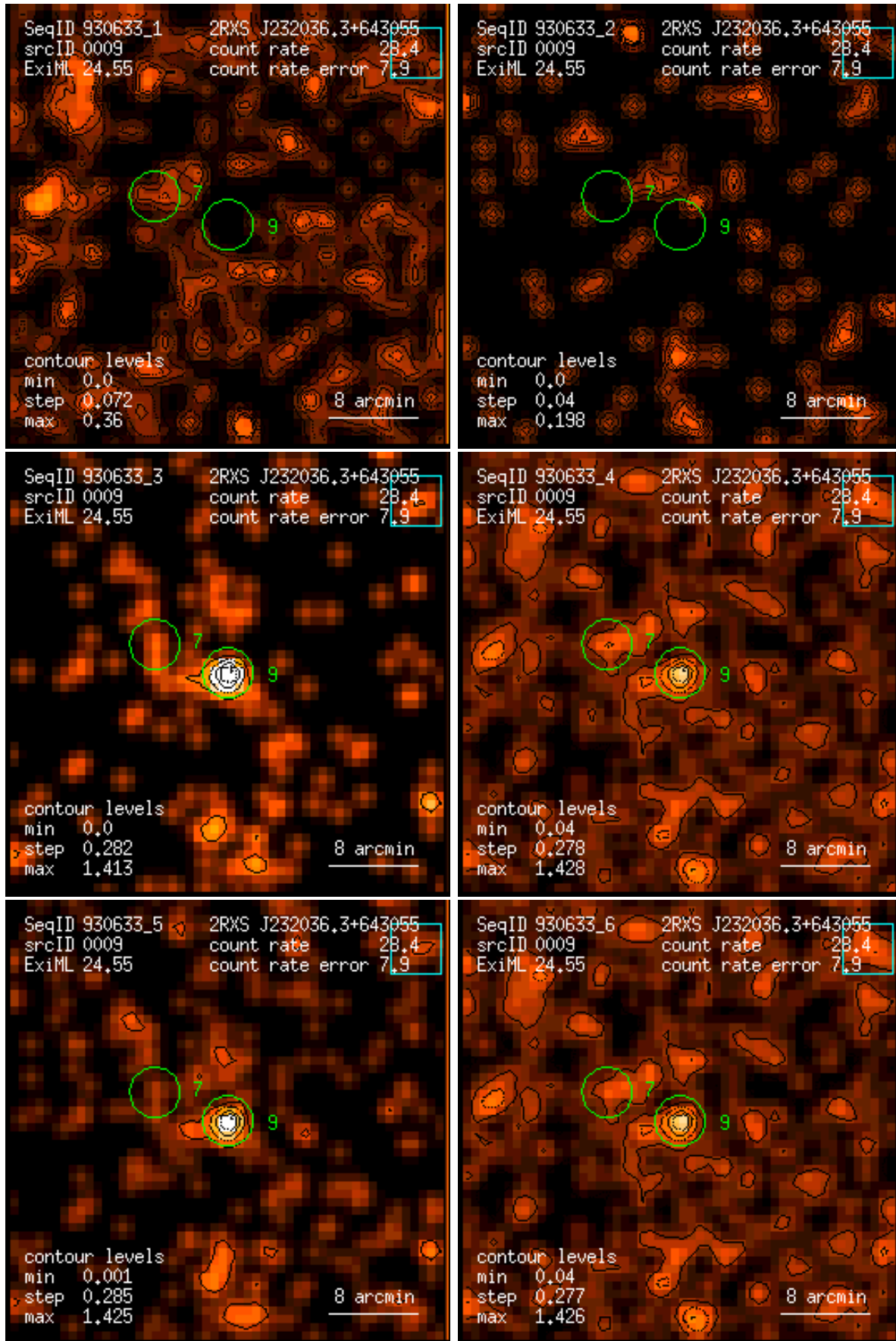
Figure 9: RASS 930633: detection 0009: band rate images, Gaussian filter: (1) PSPC channels 11 – 41, (2) 52 – 90, (3) 91 – 201, (4) 11 – 235, (5) 52 – 201, (6) 11 – 201. Broad band rates in counts/ks. Band rate contour levels in counts/ks/arcmin 2 .
